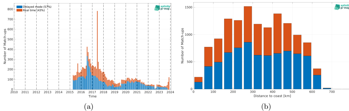
Figure 2: Number of match-ups between Argo and SMAP SSS L3 v5.3 - 8-Day running (RSS) SSS as a function of time (a) and as function of the distance to coast (b) over the Ganga and Brahmaputra river plumes Pi-MEP region and for the full satellite product period.
