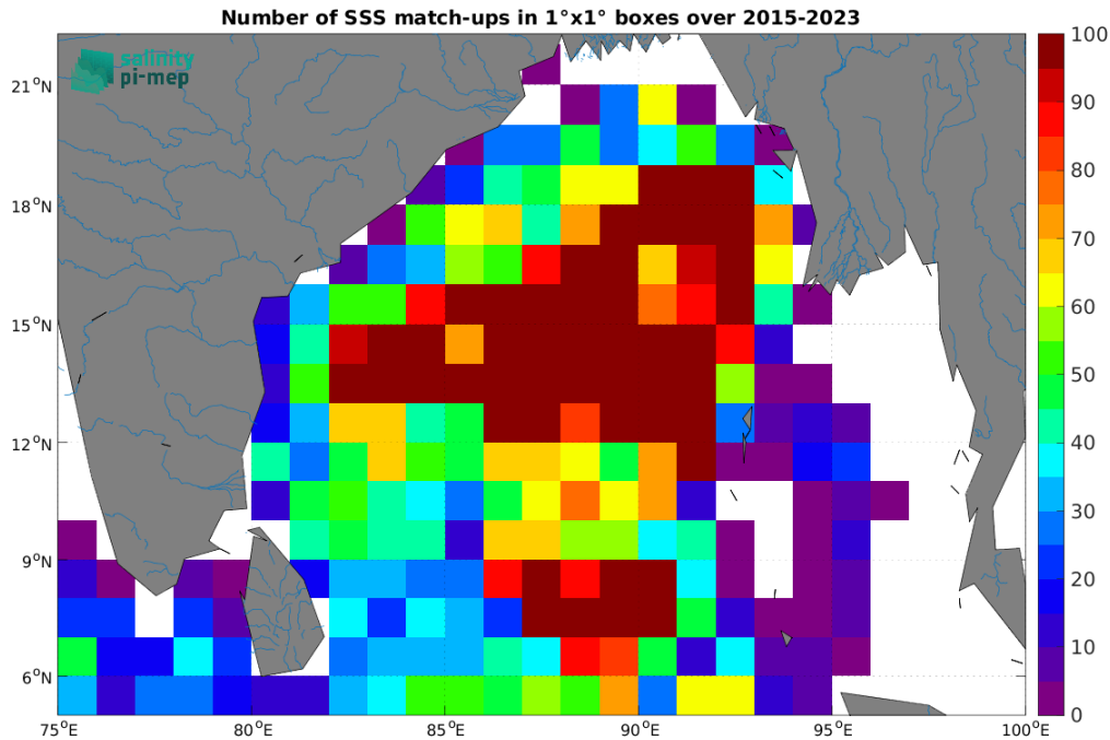
Figure 5: Number of SSS match-ups between Argo SSS and the SMAP SSS L3 v5.3 - 8-Day running (RSS) SSS product for the Ganga and Brahmaputra river plumes Pi-MEP region over 1^\circ \times 1^\circ boxes and for the full satellite product period.
