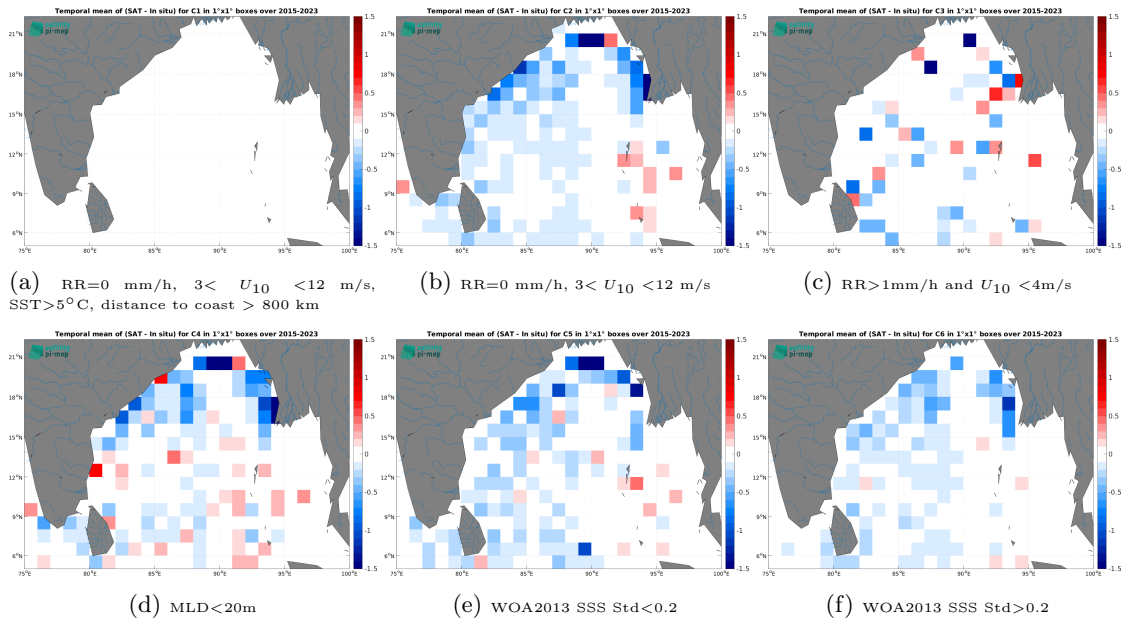
Figure 14: Temporal mean gridded over spatial boxes of size 1^\circ \times 1^\circ of \Delta SSS (SMAP SSS L3 v5.3 - 8-Day running (RSS) - Argo) for 6 different subdatasets corresponding to:RR=0 mm/h, 3 < U_{10} < 12 m/s, SST>5°C, distance to coast > 800 km (a), RR=0 mm/h, 3 < U_{10} < 12 m/s (b), RR>1mm/h and U_{10} < 4 m/s (c),MLD<20m (d),WOA2013 SSS Std<0.2 (e),WOA2013 SSS Std>0.2 (f).
