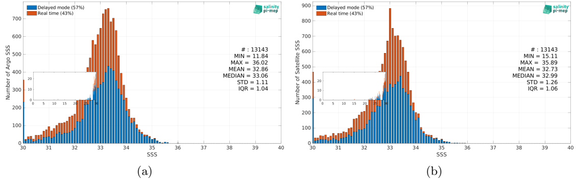
Figure 3: Histograms of SSS from Argo (a) and SMAP SSS L3 v5.3 - 8-Day running (RSS) (b) considering all match-up pairs per bins of 0.1 over the Ganga and Brahmaputra river plumes Pi-MEP region and for the full satellite product period.
