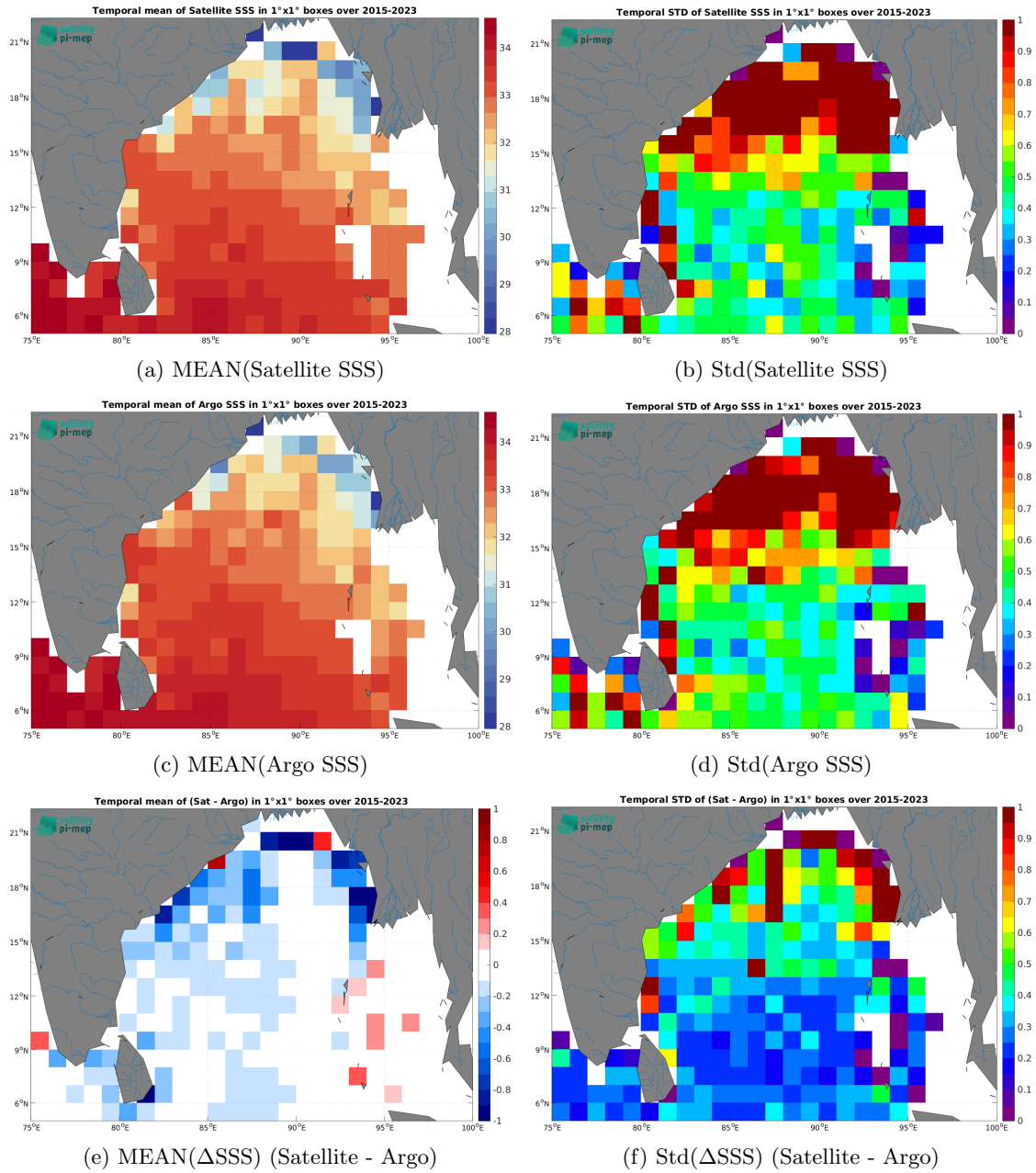
Figure 7: Temporal mean (left) and Std (right) of SSS from SMAP SSS L3 v5.3 - 8-Day running (RSS) (top), Argo (middle), and of \Delta SSS (Satellite - Argo). Only match-up pairs are used to generate these maps.
