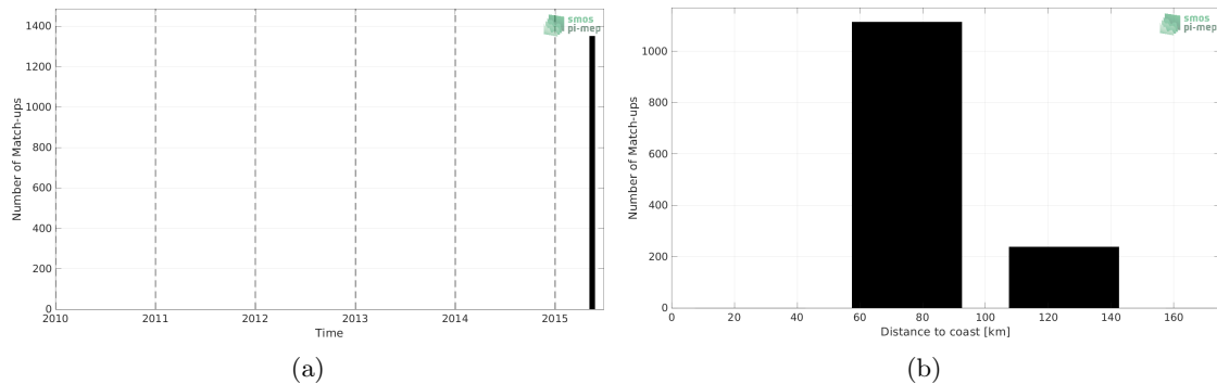
Figure 1: Number of match-ups between TSG (SAMOS) and SMAP SSS L3 v5 - 8-Day running (RSS) SSS as a function of time (a) and as function of the distance to coast (b) over the Ganga and Brahmaputra river plumes Pi-MEP region and for the full satellite product period.
