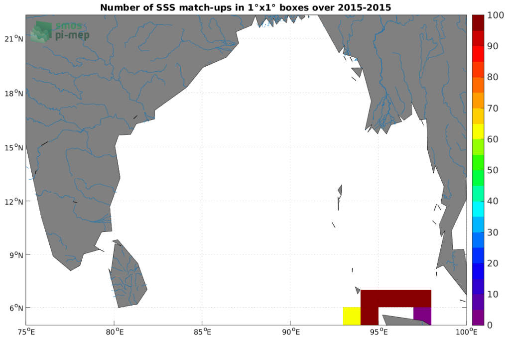
Figure 4: Number of SSS match-ups between TSG (SAMOS) SSS and the SMAP SSS L3 v5 - 8-Day running (RSS) SSS product for the Ganga and Brahmaputra river plumes Pi-MEP region over 1°x1° boxes and for the full satellite product period.
