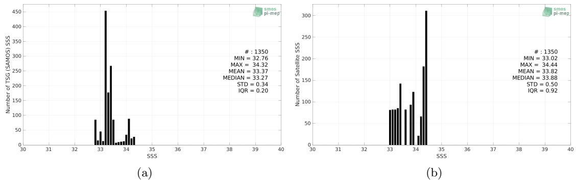
Figure 2: Histograms of SSS from TSG (SAMOS) (a) and SMAP SSS L3 v5 - 8-Day running (RSS) (b) considering all match-up pairs per bins of 0.1 over the Ganga and Brahmaputra river plumes Pi-MEP region and for the full satellite product period.
