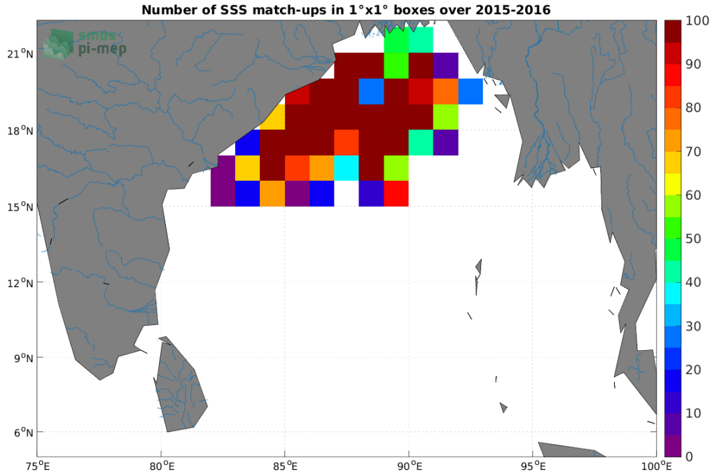
Figure 3: Number of SSS match-ups between Surface drifters SSS and the SMAP SSS L3 v5 - 8-Day running (RSS) SSS product for the Ganga and Brahmaputra river plumes Pi-MEP region over 1^\circ \times 1^\circ boxes and for the full satellite product period.
