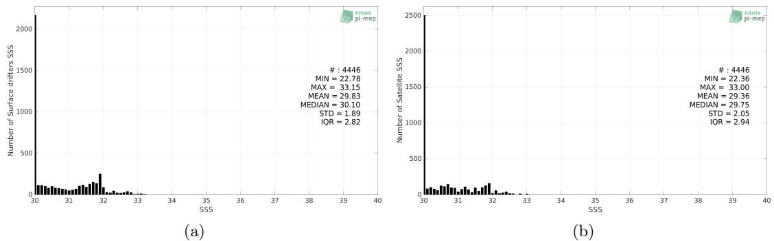
Figure 2: Histograms of SSS from Surface drifters (a) and SMAP SSS L3 v5 - 8-Day running (RSS) (b) considering all match-up pairs per bins of 0.1 over the Ganga and Brahmaputra river plumes Pi-MEP region and for the full satellite product period.
