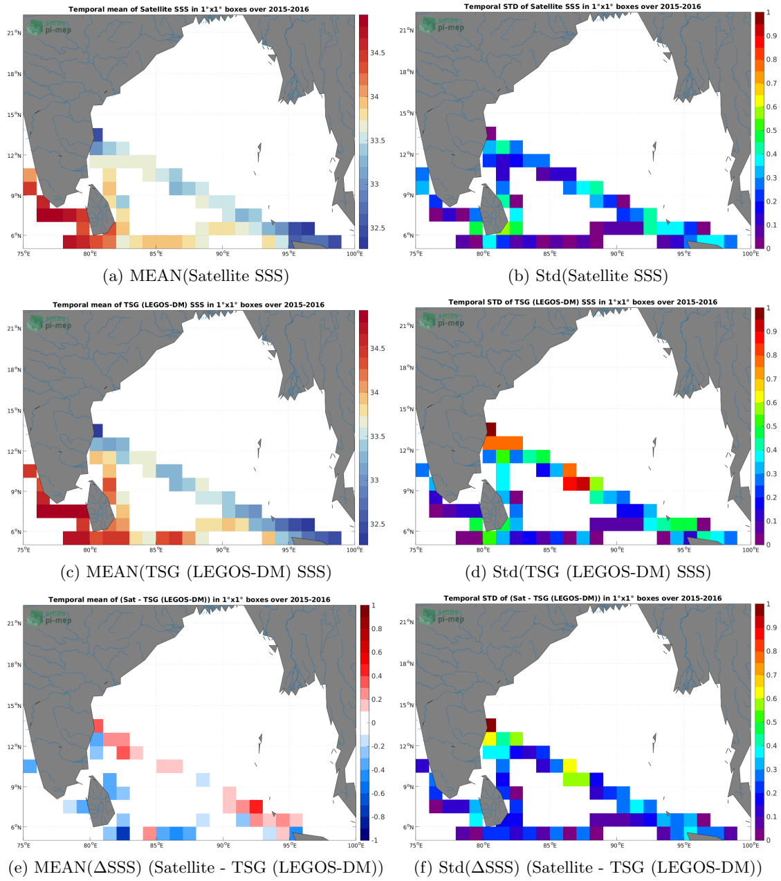
Figure 6: Temporal mean (left) and Std (right) of SSS from SMAP SSS L3 v5 - Monthly (RSS) (top), TSG (LEGOS-DM) (middle), and of \Delta SSS (Satellite - TSG (LEGOS-DM)). Only match-pairs are used to generate these maps.
