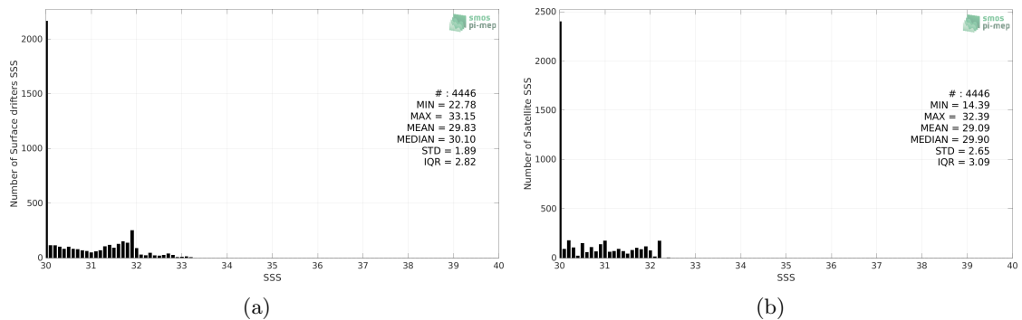
Figure 2: Histograms of SSS from Surface drifters (a) and SMAP SSS L3 v5 - Monthly (RSS) (b) considering all match-up pairs per bins of 0.1 over the Ganga and Brahmaputra river plumes Pi-MEP region and for the full satellite product period.
