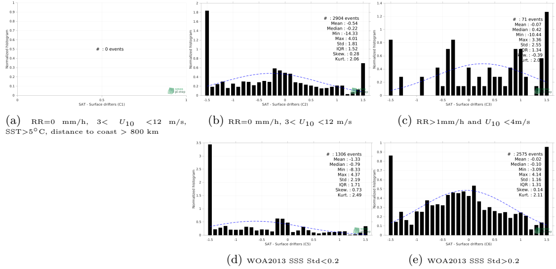
Figure 12: Normalized histogram of \Delta SSS (SMAP SSS L3 v5 - Monthly (RSS) - Surface drifters) for 5 different subdatasets corresponding to: RR=0 mm/h, 3 < U_{10} < 12 m/s, SST > 5°C, distance to coast > 800 km (a), RR=0 mm/h, 3 < U_{10} < 12 m/s (b), RR > 1mm/h and U_{10} < 4 m/s (c), WOA2013 SSS Std < 0.2 (d), WOA2013 SSS Std > 0.2 (e).
