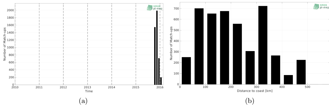
Figure 1: Number of match-ups between Surface drifters and SMAP SSS L3 v5 - Monthly (RSS) SSS as a function of time (a) and as function of the distance to coast (b) over the Ganga and Brahmaputra river plumes Pi-MEP region and for the full satellite product period.
