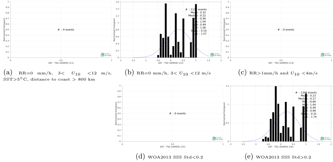
Figure 13: Normalized histogram of \Delta\text{SSS} (SMAP SSS L3 v4 - 8-Day running (RSS) - TSG (SAMOS)) for 5 different subdatasets corresponding to: RR=0 mm/h, 3 < U_{10} < 12 m/s, SST > 5^\circ\text{C} , distance to coast > 800 km (a), RR=0 mm/h, 3 < U_{10} < 12 m/s (b), RR > 1 mm/h and U_{10} < 4 m/s (c), WOA2013 SSS Std < 0.2 (d), WOA2013 SSS Std > 0.2 (e).
