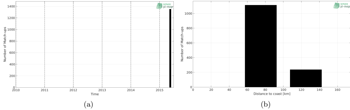
Figure 1: Number of match-ups between TSG-SAMOS and SMAP-L3-RSS-V4-8DAY-RUNNING SSS as a function of time (a) and as function of the distance to coast (b) over the Ganga and Brahmaputra river plumes Pi-MEP region and for the full satellite product period.
