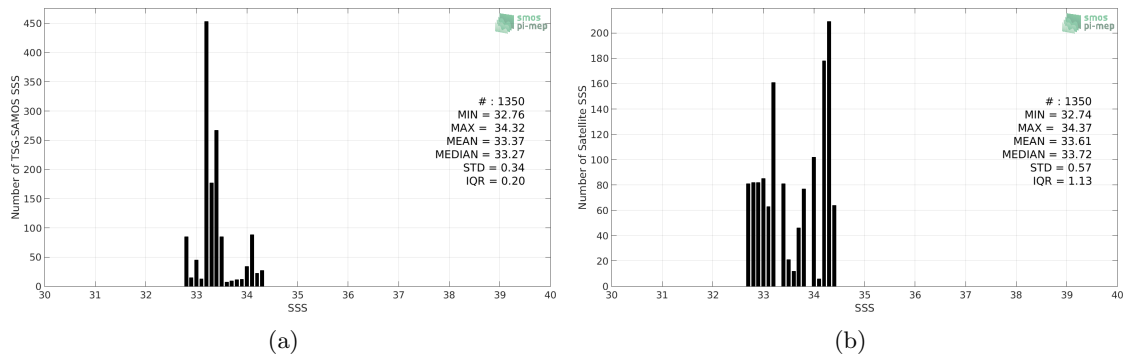
Figure 2: Histograms of SSS from TSG-SAMOS (a) and SMAP-L3-RSS-V4-8DAY-RUNNING (b) considering all match-up pairs per bins of 0.1 over the Ganga and Brahmaputra river plumes Pi-MEP region and for the full satellite product period.
