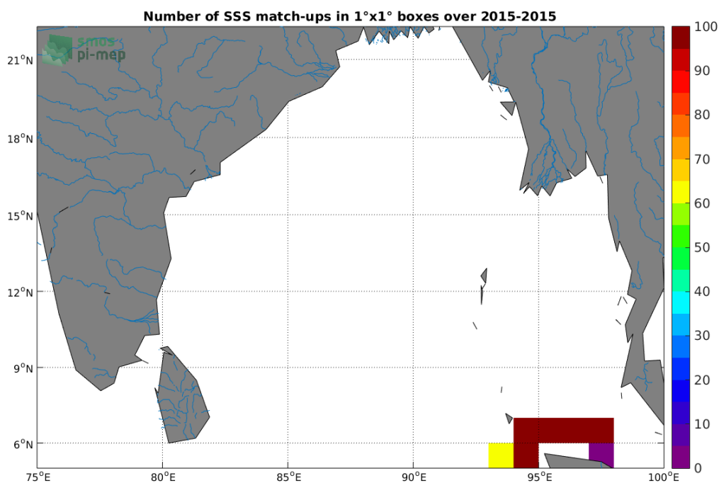
Figure 4: Number of SSS match-ups between TSG-SAMOS SSS and the SMAP-L3-RSS-V4-8DAY-RUNNING SSS product for the Ganga and Brahmaputra river plumes Pi-MEP region over 1^\circ \times 1^\circ boxes and for the full satellite product period.
