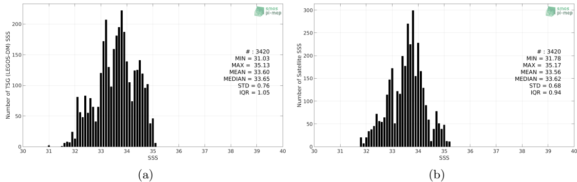
Figure 2: Histograms of SSS from TSG (LEGOS-DM) (a) and SMAP SSS L3 v4 - 8-Day running (RSS) (b) considering all match-up pairs per bins of 0.1 over the Ganga and Brahmaputra river plumes Pi-MEP region and for the full satellite product period.
