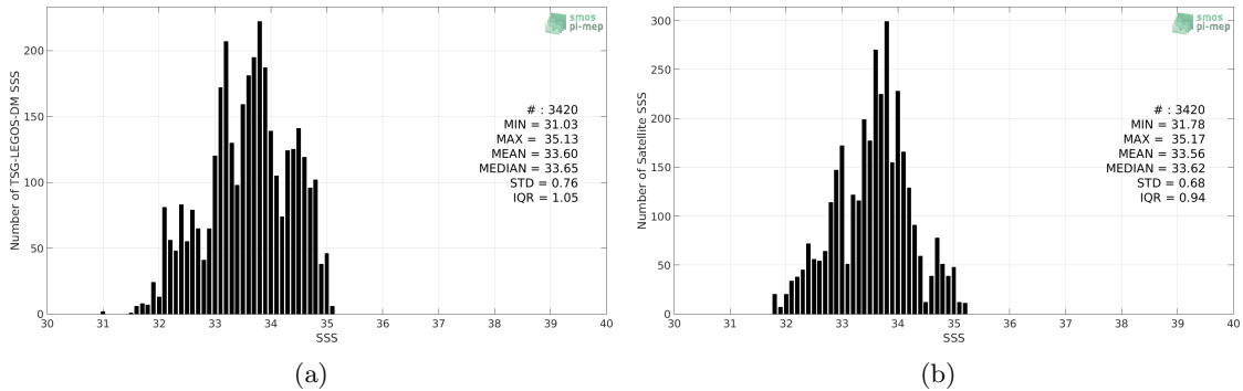
Figure 2: Histograms of SSS from TSG-LEGOS-DM (a) and SMAP-L3-RSS-V4-8DAY-RUNNING (b) considering all match-up pairs per bins of 0.1 over the Ganga and Brahmaputra river plumes Pi-MEP region and for the full satellite product period.
