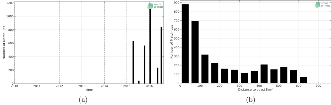
Figure 1: Number of match-ups between TSG-LEGOS-DM and SMAP-L3-RSS-V4-8DAY-RUNNING SSS as a function of time (a) and as function of the distance to coast (b) over the Ganga and Brahmaputra river plumes Pi-MEP region and for the full satellite product period.
