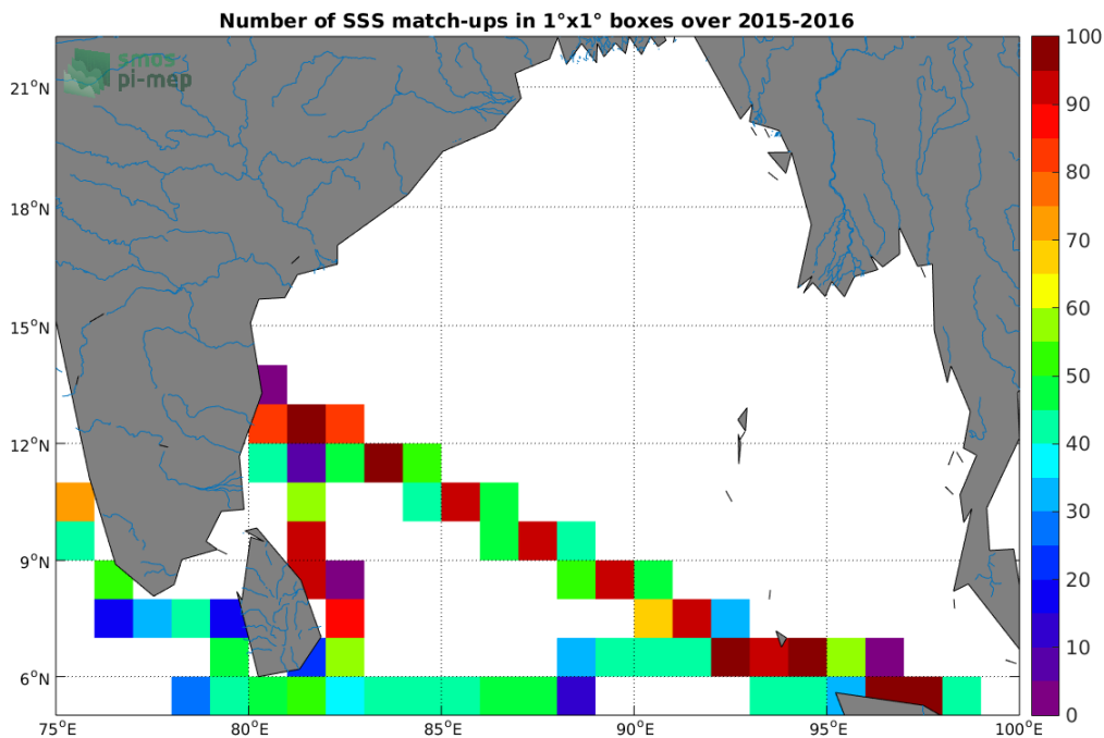
Figure 4: Number of SSS match-ups between TSG-LEGOS-DM SSS and the SMAP-L3-RSS-V4-8DAY-RUNNING SSS product for the Ganga and Brahmaputra river plumes Pi-MEP region over 1°x1° boxes and for the full satellite product period.
