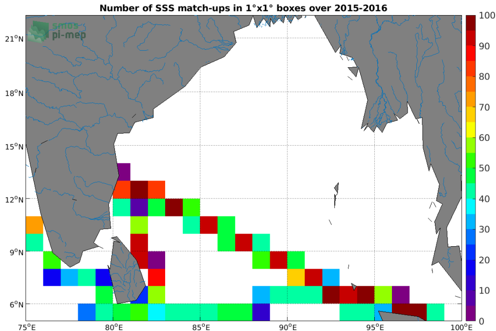
Figure 4: Number of SSS match-ups between TSG (LEGOS-DM) SSS and the SMAP SSS L3 v4 - Monthly (RSS) SSS product for the Ganga and Brahmaputra river plumes Pi-MEP region over 1^{\circ} \times 1^{\circ} boxes and for the full satellite product period.
