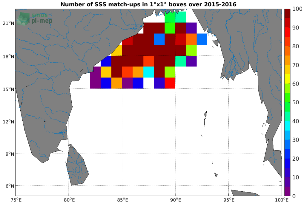
Figure 3: Number of SSS match-ups between Surface drifters SSS and the SMAP SSS L3 v4 - Monthly (RSS) SSS product for the Ganga and Brahmaputra river plumes Pi-MEP region over 1^{\circ} \times 1^{\circ} boxes and for the full satellite product period.
