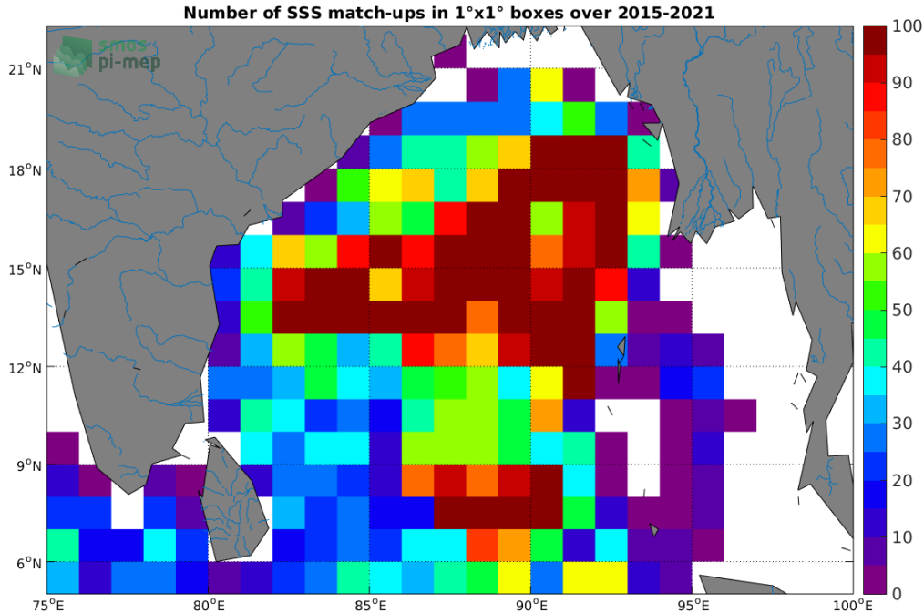
Figure 4: Number of SSS match-ups between Argo SSS and the SMAP SSS L3 v4 - Monthly (RSS) SSS product for the Ganga and Brahmaputra river plumes Pi-MEP region over 1^\circ \times 1^\circ boxes and for the full satellite product period.
