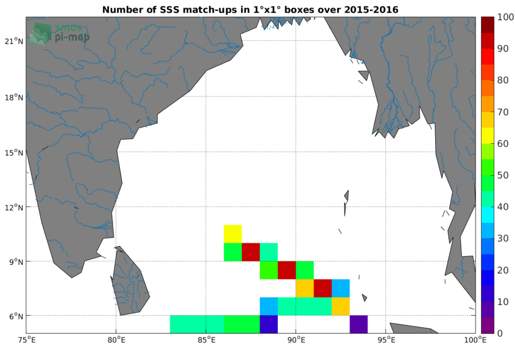
Figure 4: Number of SSS match-ups between TSG-LEGOS-DM SSS and the SMAP-L3-RSS-V3-8DAY-RUNNING-70KM SSS product for the Ganga and Brahmaputra river plumes Pi-MEP region over 1^{\circ} \times 1^{\circ} boxes and for the full satellite product period.
