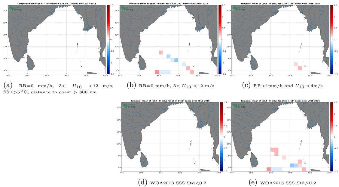
Figure 12: Temporal mean gridded over spatial boxes of size 1^\circ \times 1^\circ of \Delta SSS (SMAP-L3-RSS-V3-8DAY-RUNNING-70KM - TSG-LEGOS-DM) for 5 different subdatasets corresponding to:RR=0 mm/h, 3 < U_{10} < 12 m/s, SST > 5^\circ\text{C} , distance to coast > 800 km (a), RR=0 mm/h, 3 < U_{10} < 12 m/s (b), RR > 1 mm/h and U_{10} < 4 m/s (c), WOA2013 SSS Std < 0.2 (d), WOA2013 SSS Std > 0.2 (e).
