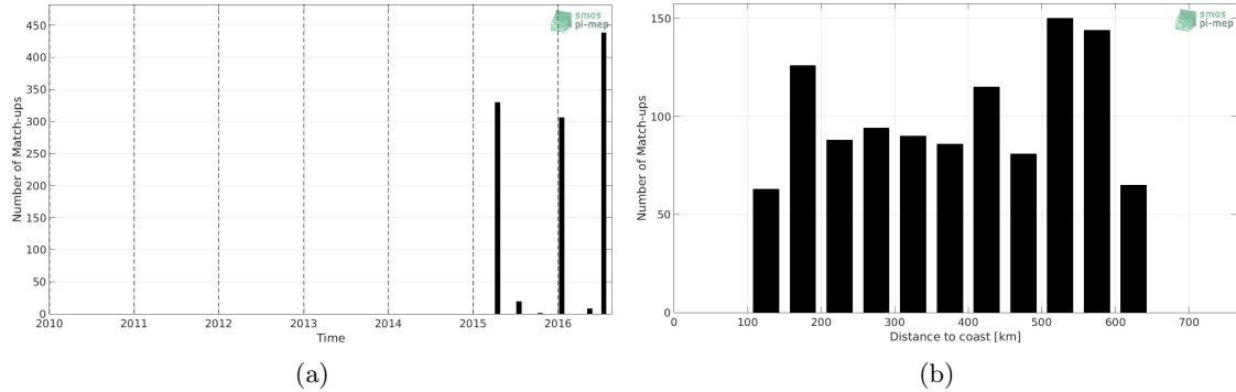
Figure 1: Number of match-ups between TSG-LEGOS-DM and SMAP-L3-RSS-V3-8DAY-RUNNING-70KM SSS as a function of time (a) and as function of the distance to coast (b) over the Ganga and Brahmaputra river plumes Pi-MEP region and for the full satellite product period.
