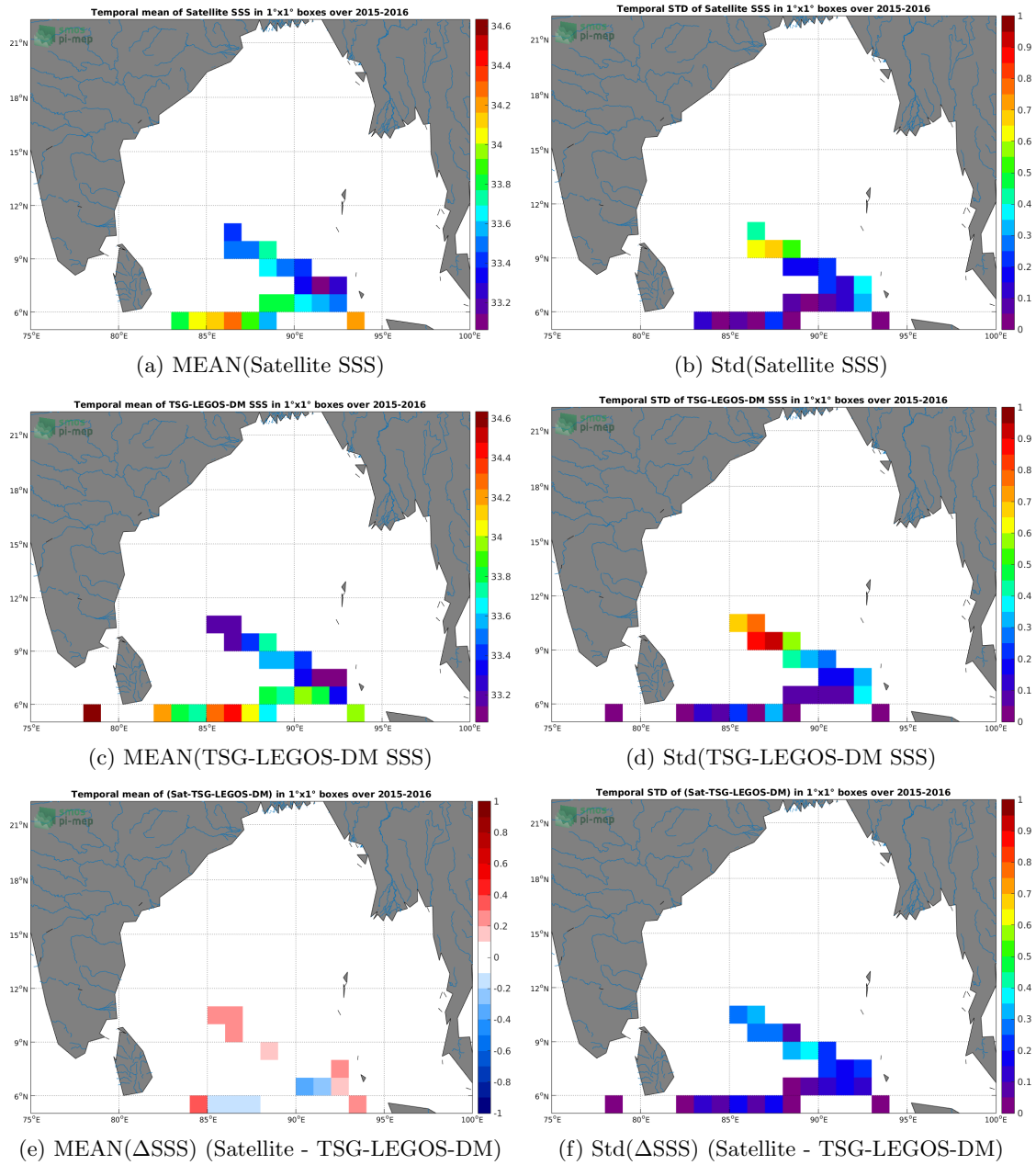
Figure 6: Temporal mean (left) and Std (right) of SSS from SMAP-L3-RSS-V3-8DAY-RUNNING-70KM (top), TSG-LEGOS-DM (middle), and of \Delta SSS (Satellite - TSG-LEGOS-DM). Only match-up pairs are used to generate these maps.
