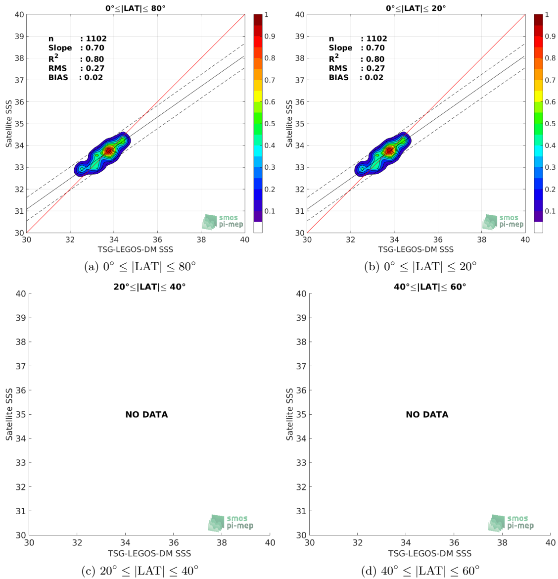
Figure 9: Contour maps of the concentration of SMAP-L3-RSS-V3-8DAY-RUNNING-70KM SSS (y-axis) versus TSG-LEGOS-DM SSS (x-axis) at match-up pairs for different latitude bands. For each plot, the red line shows x=y . The black thin and dashed lines indicate a linear fit through the data cloud and the \pm 95\% confidence levels, respectively. The number match-up pairs n , the slope and R^2 coefficient of the linear fit, the root mean square (RMS) and the mean bias between satellite and in situ data are indicated for each latitude band in each plots.
