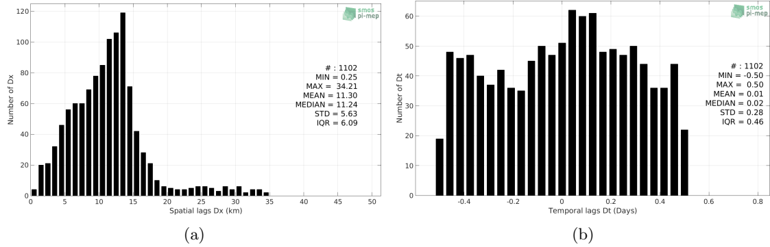
Figure 5: Histograms of the spatial (a) and temporal (b) lags between the time of the TSG-LEGOS-DM measurements and the date of the corresponding SMAP-L3-RSS-V3-8DAY-RUNNING-70KM SSS product.
