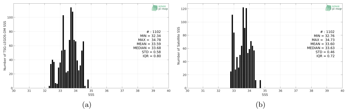
Figure 2: Histograms of SSS from TSG-LEGOS-DM (a) and SMAP-L3-RSS-V3-8DAY-RUNNING-70KM (b) considering all match-up pairs per bins of 0.1 over the Ganga and Brahmaputra river plumes Pi-MEP region and for the full satellite product period.
