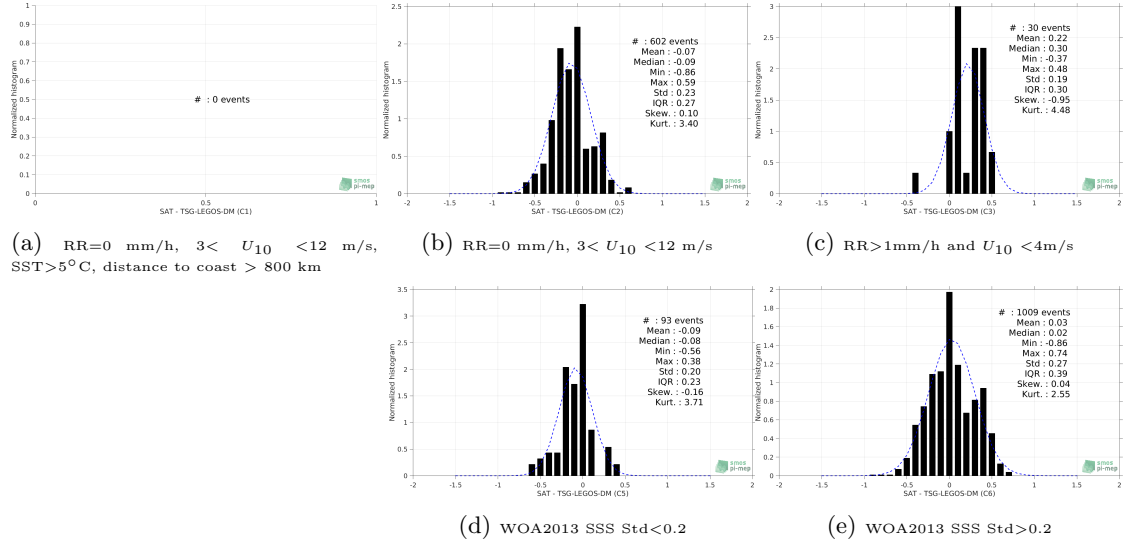
Figure 13: Normalized histogram of \Delta SSS (SMAP-L3-RSS-V3-8DAY-RUNNING-70KM - TSG-LEGOS-DM) for 5 different subdatasets corresponding to: RR=0 mm/h, 3 < U_{10} < 12 m/s, SST > 5°C, distance to coast > 800 km (a), RR=0 mm/h, 3 < U_{10} < 12 m/s (b), RR > 1mm/h and U_{10} < 4 m/s (c), WOA2013 SSS Std < 0.2 (d), WOA2013 SSS Std > 0.2 (e).
