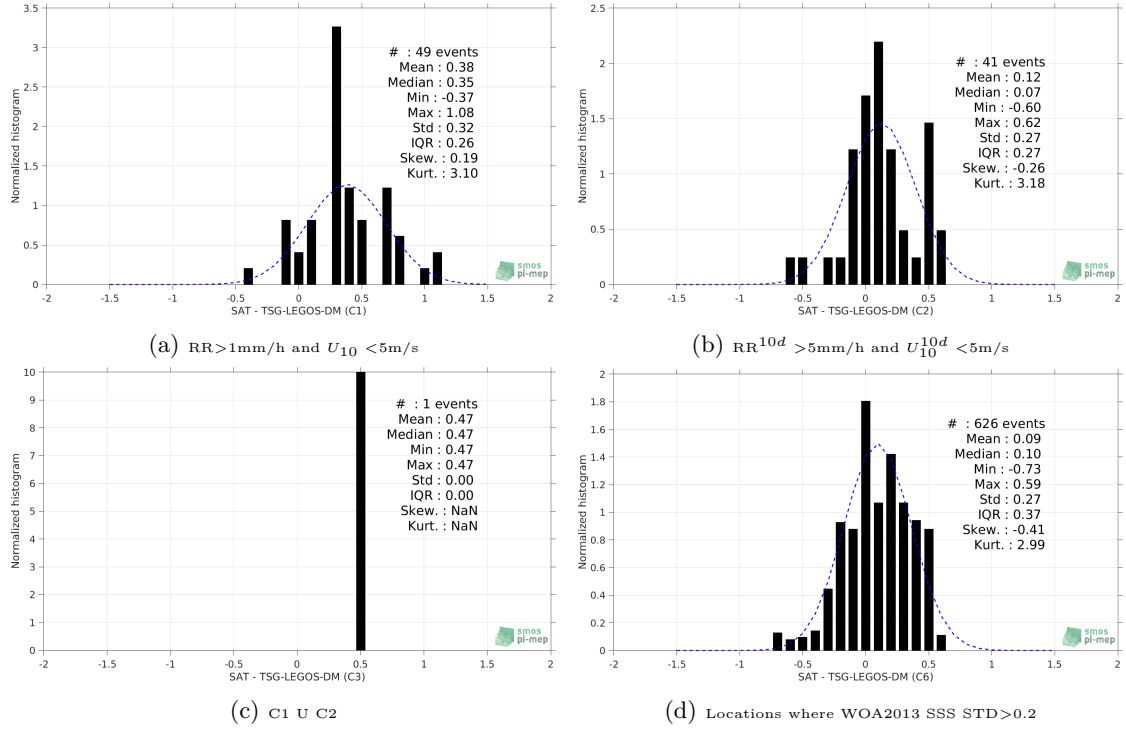
Figure 13: Normalized histogram of \Delta SSS (SMAP-L3-RSS-V3-8DAY-RUNNING-70KM - TSG-LEGOS-DM) for 6 different subdatasets corresponding to: RR > 1\text{mm/h} and U_{10} < 5\text{m/s} (a), RR^{10d} > 5\text{mm/h} and U_{10}^{10d} < 5\text{m/s} (b), C1 U C2 (c), Locations where WOA2013 SSS STD > 0.2 (d).
