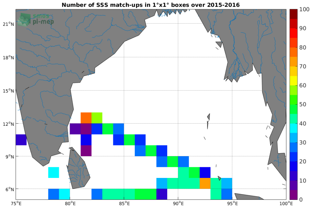
Figure 4: Number of SSS match-ups between TSG-LEGOS-DM SSS and the SMAP-L3-RSS-V3-8DAY-RUNNING-70KM SSS product for the Ganga and Brahmaputra river plumes Pi-MEP region over 1°x1° boxes and for the full satellite product period.
