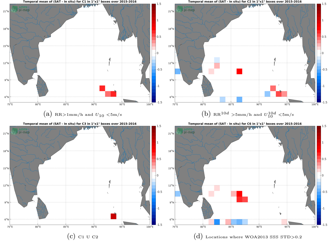
Figure 12: Temporal mean gridded over spatial boxes of size 1^\circ \times 1^\circ of \Delta SSS (SMAP-L3-RSS-V3-MONTHLY-70KM - TSG-LEGOS-DM) for 4 different subdatasets corresponding to: RR > 1mm/h and U_{10} < 5\text{m/s} (a), RR^{10d} > 5\text{mm/h} and U_{10}^{10d} < 5\text{m/s} (b), C1 U C2 (c), Locations where WOA2013 SSS STD > 0.2 (d).
