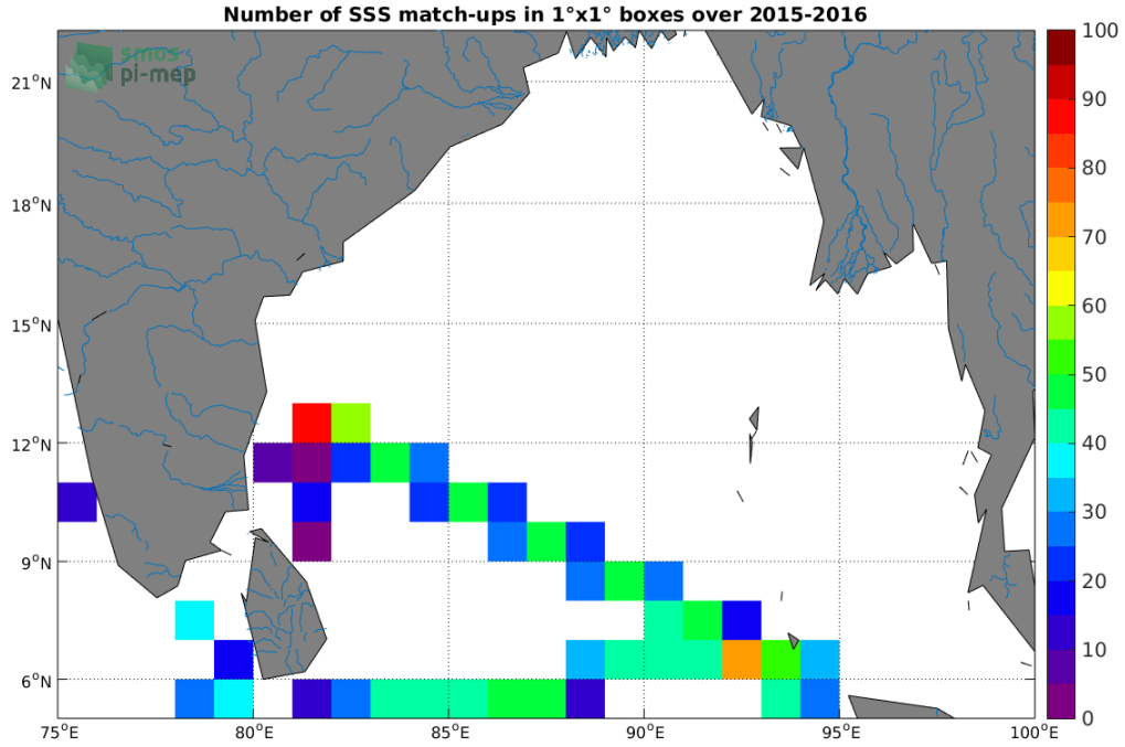
Figure 4: Number of SSS match-ups between TSG-LEGOS-DM SSS and the SMAP-L3-RSS-V3-MONTHLY-70KM SSS product for the Ganga and Brahmaputra river plumes Pi-MEP region over 1^\circ \times 1^\circ boxes and for the full satellite product period.
