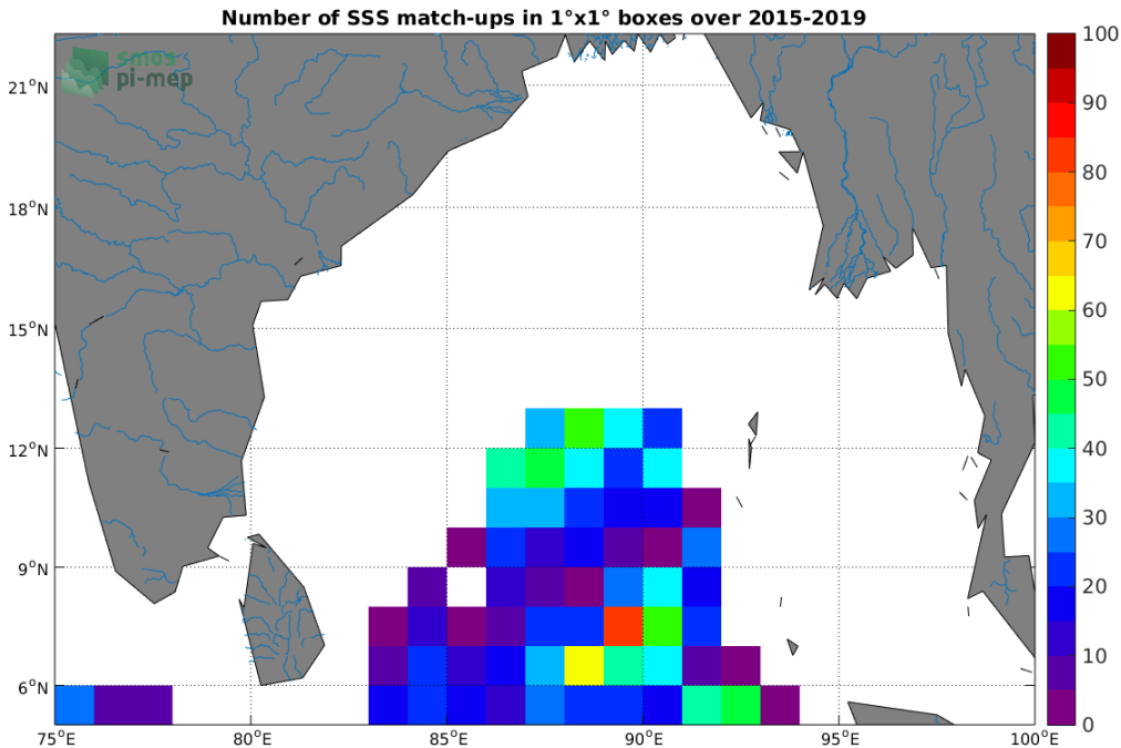
Figure 4: Number of SSS match-ups between Argo SSS and the SMAP-L3-RSS-V3-MONTHLY-70KM SSS product for the Ganga and Brahmaputra river plumes Pi-MEP region over 1^\circ \times 1^\circ boxes and for the full satellite product period.
