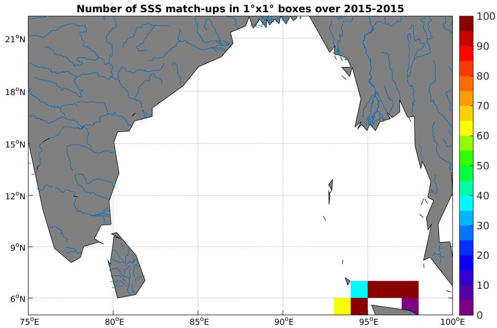
Figure 4: Number of SSS match-ups between TSG-SAMOS SSS and the SMAP-L3-RSS-V2-8DAY-RUNNING-70KM SSS product for the Ganga and Brahmaputra river plumes Pi-MEP region over 1^\circ \times 1^\circ boxes and for the full satellite product period.
