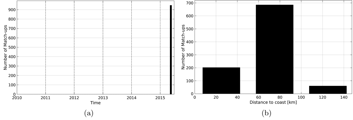
Figure 1: Number of match-ups between TSG-SAMOS and SMAP-L3-RSS-V2-8DAY-RUNNING-70KM SSS as a function of time (a) and as function of the distance to coast (b) over the Ganga and Brahmaputra river plumes Pi-MEP region and for the full satellite product period.
