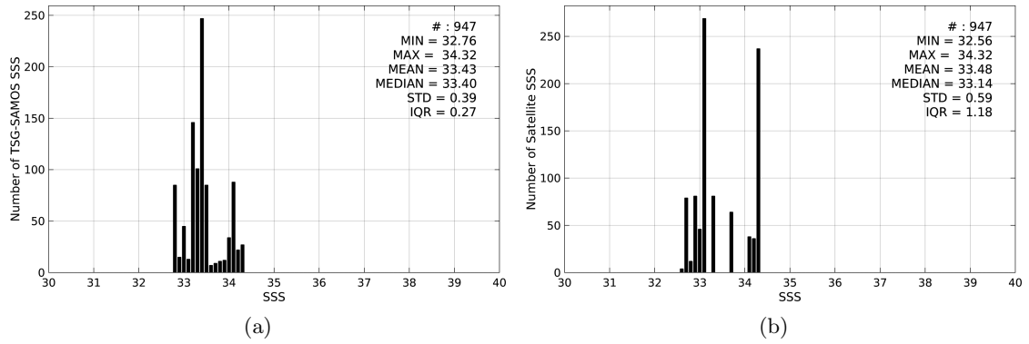
Figure 2: Histograms of SSS from TSG-SAMOS (a) and SMAP-L3-RSS-V2-8DAY-RUNNING-70KM (b) considering all match-up pairs per bins of 0.1 over the Ganga and Brahmaputra river plumes Pi-MEP region and for the full satellite product period.
