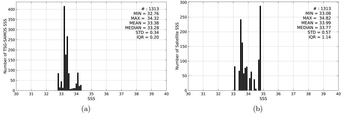
Figure 2: Histograms of SSS from TSG-SAMOS (a) and SMAP-L3-RSS-V2-MONTHLY-0.25DEG-40KM (b) considering all match-up pairs per bins of 0.1 over the Ganga and Brahmaputra river plumes Pi-MEP region and for the full satellite product period.
