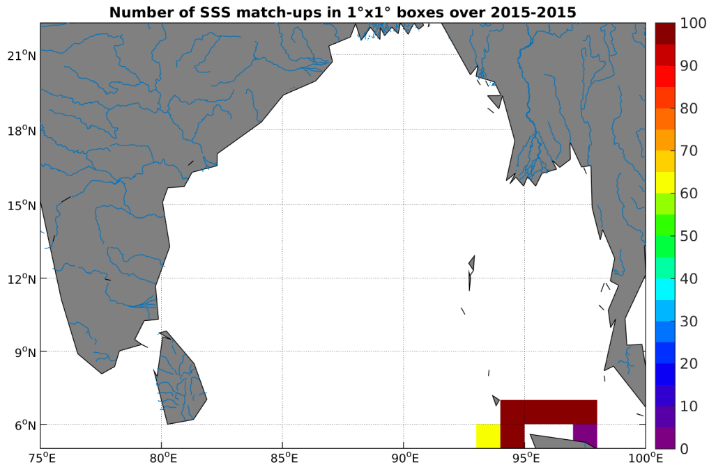
Figure 4: Number of SSS match-ups between TSG-SAMOS SSS and the SMAP-L3-RSS-V2-MONTHLY-0.25DEG-40KM SSS product for the Ganga and Brahmaputra river plumes Pi-MEP region over 1^\circ \times 1^\circ boxes and for the full satellite product period.
