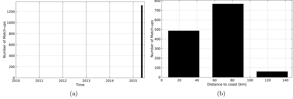
Figure 1: Number of match-ups between TSG-SAMOS and SMAP-L3-RSS-V2-MONTHLY-0.25DEG-40KM SSS as a function of time (a) and as function of the distance to coast (b) over the Ganga and Brahmaputra river plumes Pi-MEP region and for the full satellite product period.
