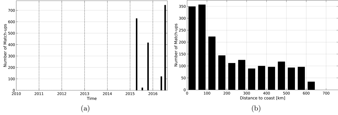
Figure 1: Number of match-ups between TSG-LEGOS-DM and SMAP-L3-RSS-V2-MONTHLY-0.25DEG-40KM SSS as a function of time (a) and as function of the distance to coast (b) over the Ganga and Brahmaputra river plumes Pi-MEP region and for the full satellite product period.
