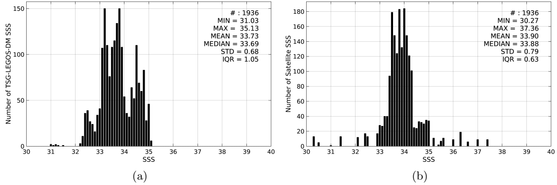
Figure 2: Histograms of SSS from TSG-LEGOS-DM (a) and SMAP-L3-RSS-V2-MONTHLY-0.25DEG-40KM (b) considering all match-up pairs per bins of 0.1 over the Ganga and Brahmaputra river plumes Pi-MEP region and for the full satellite product period.
