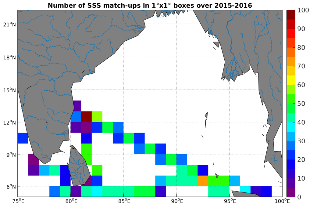
Figure 4: Number of SSS match-ups between TSG-LEGOS-DM SSS and the SMAP-L3-RSS-V2-MONTHLY-0.25DEG-40KM SSS product for the Ganga and Brahmaputra river plumes Pi-MEP region over 1^\circ \times 1^\circ boxes and for the full satellite product period.
