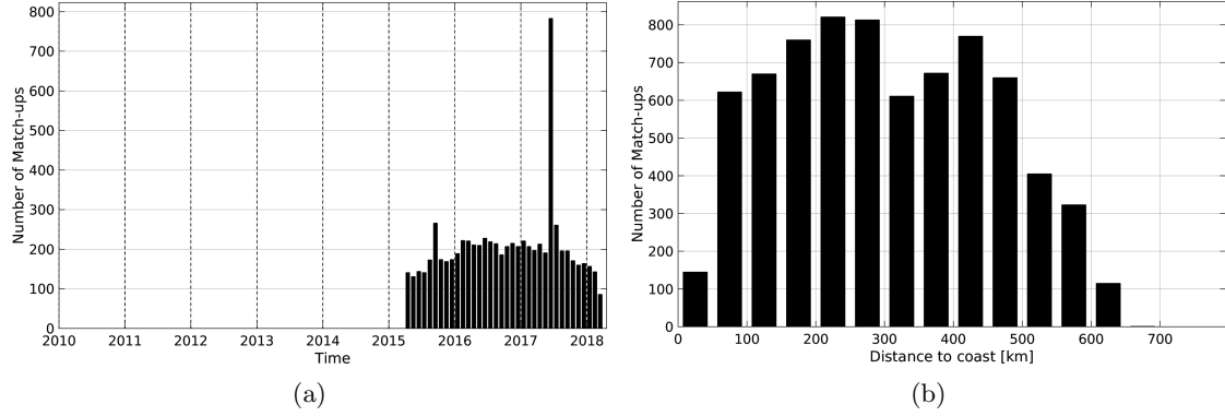
Figure 1: Number of match-ups between Argo and SMAP-L3-RSS-V2-MONTHLY-0.25DEG-40KM SSS as a function of time (a) and as function of the distance to coast (b) over the Ganga and Brahmaputra river plumes Pi-MEP region and for the full satellite product period.
