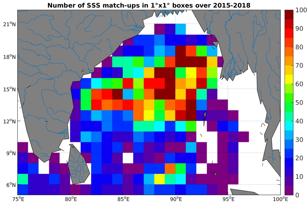
Figure 4: Number of SSS match-ups between Argo SSS and the SMAP-L3-RSS-V2-MONTHLY-0.25DEG-40KM SSS product for the Ganga and Brahmaputra river plumes Pi-MEP region over 1^\circ \times 1^\circ boxes and for the full satellite product period.
