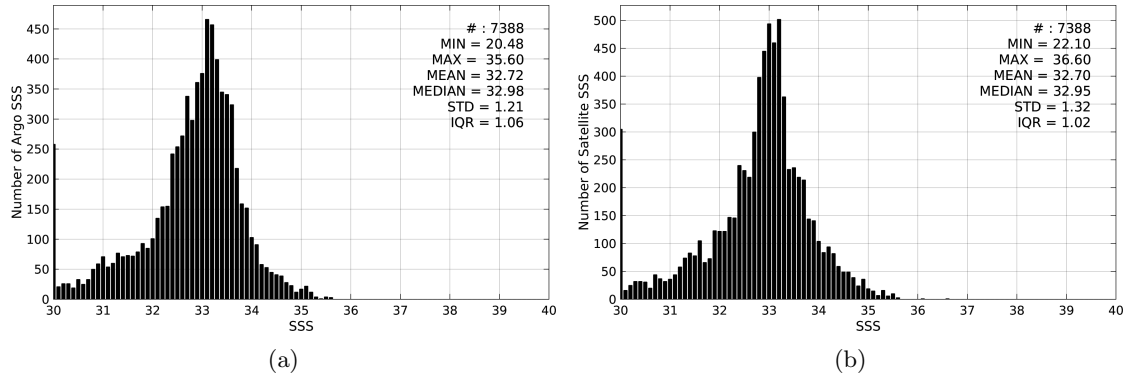
Figure 2: Histograms of SSS from Argo (a) and SMAP-L3-RSS-V2-MONTHLY-0.25DEG-40KM (b) considering all match-up pairs per bins of 0.1 over the Ganga and Brahmaputra river plumes Pi-MEP region and for the full satellite product period.
