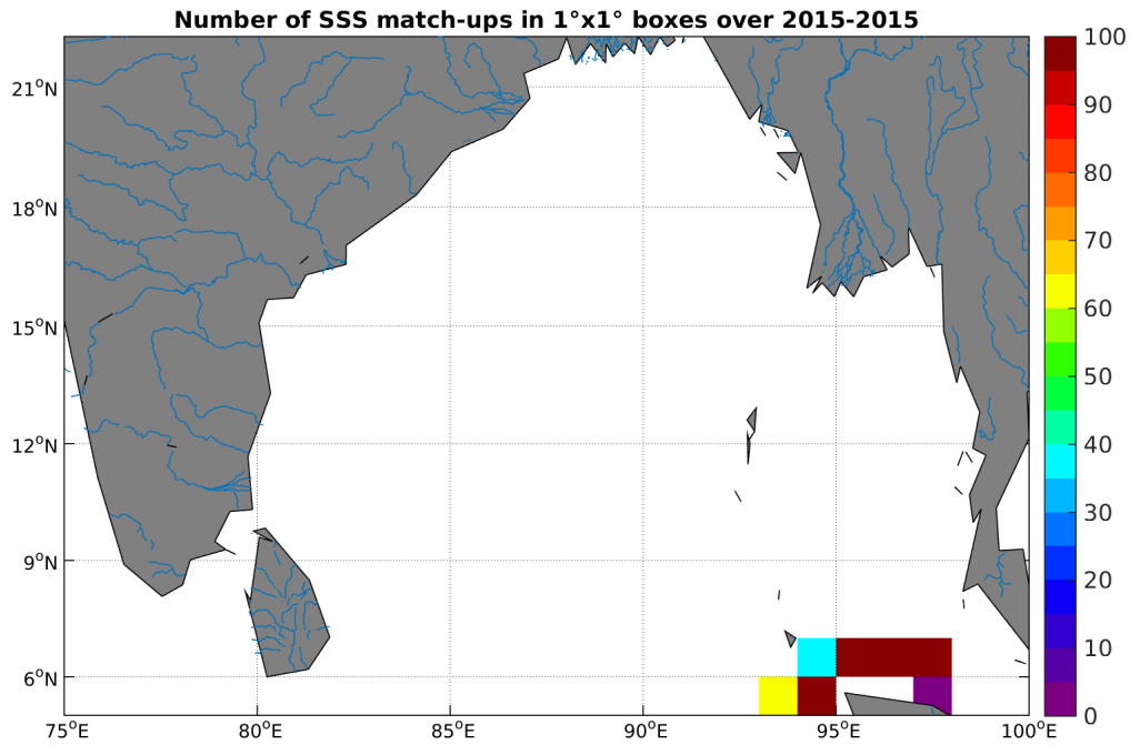
Figure 4: Number of SSS match-ups between TSG-SAMOS SSS and the SMAP-L3-RSS-V2-MONTHLY-70KM SSS product for the Ganga and Brahmaputra river plumes Pi-MEP region over 1^\circ \times 1^\circ boxes and for the full satellite product period.
