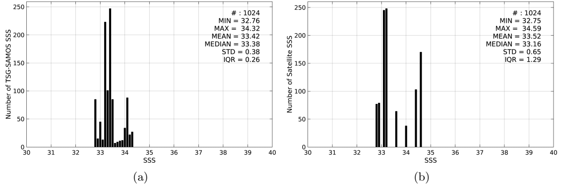
Figure 2: Histograms of SSS from TSG-SAMOS (a) and SMAP-L3-RSS-V2-MONTHLY-70KM (b) considering all match-up pairs per bins of 0.1 over the Ganga and Brahmaputra river plumes Pi-MEP region and for the full satellite product period.
