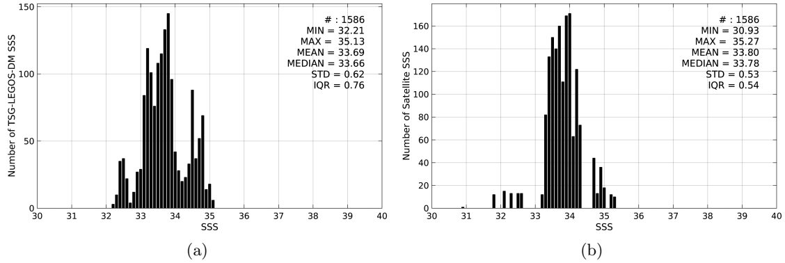
Figure 2: Histograms of SSS from TSG-LEGOS-DM (a) and SMAP-L3-RSS-V2-MONTHLY-70KM (b) considering all match-up pairs per bins of 0.1 over the Ganga and Brahmaputra river plumes Pi-MEP region and for the full satellite product period.
