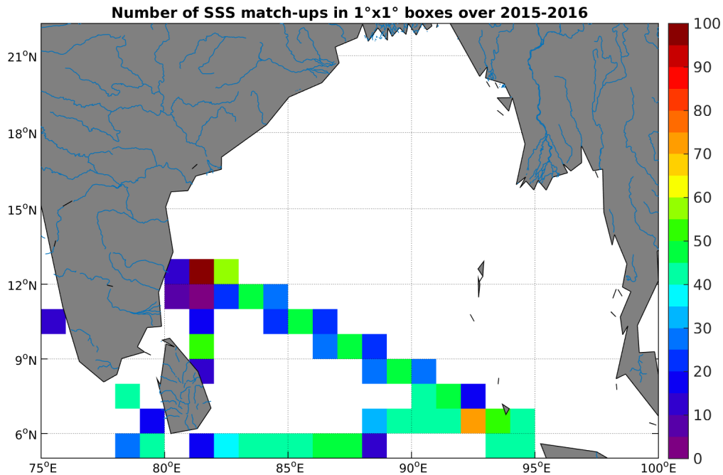
Figure 4: Number of SSS match-ups between TSG-LEGOS-DM SSS and the SMAP-L3-RSS-V2-MONTHLY-70KM SSS product for the Ganga and Brahmaputra river plumes Pi-MEP region over 1^\circ \times 1^\circ boxes and for the full satellite product period.
