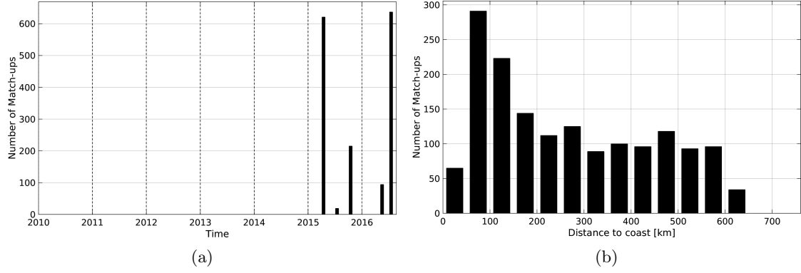
Figure 1: Number of match-ups between TSG-LEGOS-DM and SMAP-L3-RSS-V2-MONTHLY-70KM SSS as a function of time (a) and as function of the distance to coast (b) over the Ganga and Brahmaputra river plumes Pi-MEP region and for the full satellite product period.
