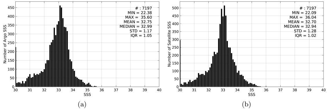
Figure 2: Histograms of SSS from Argo (a) and SMAP-L3-RSS-V2-MONTHLY-70KM (b) considering all match-up pairs per bins of 0.1 over the Ganga and Brahmaputra river plumes Pi-MEP region and for the full satellite product period.
