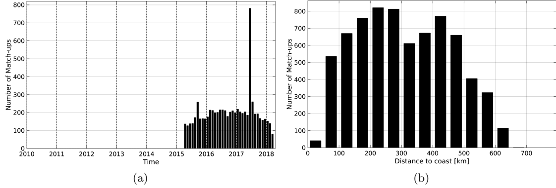
Figure 1: Number of match-ups between Argo and SMAP-L3-RSS-V2-MONTHLY-70KM SSS as a function of time (a) and as function of the distance to coast (b) over the Ganga and Brahmaputra river plumes Pi-MEP region and for the full satellite product period.
