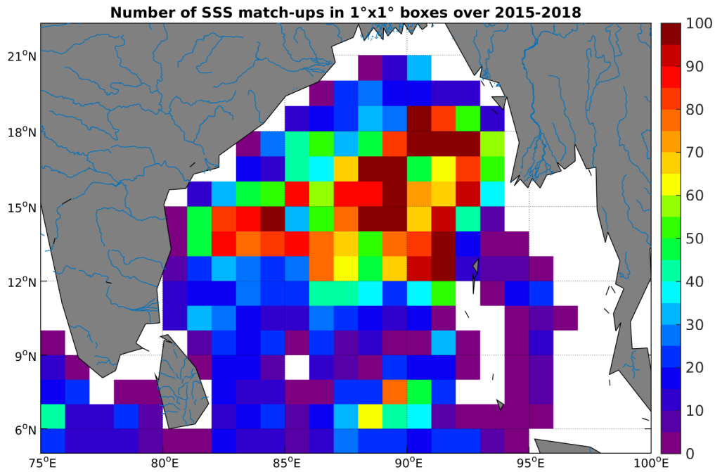
Figure 4: Number of SSS match-ups between Argo SSS and the SMAP-L3-RSS-V2-MONTHLY-70KM SSS product for the Ganga and Brahmaputra river plumes Pi-MEP region over 1°x1° boxes and for the full satellite product period.
