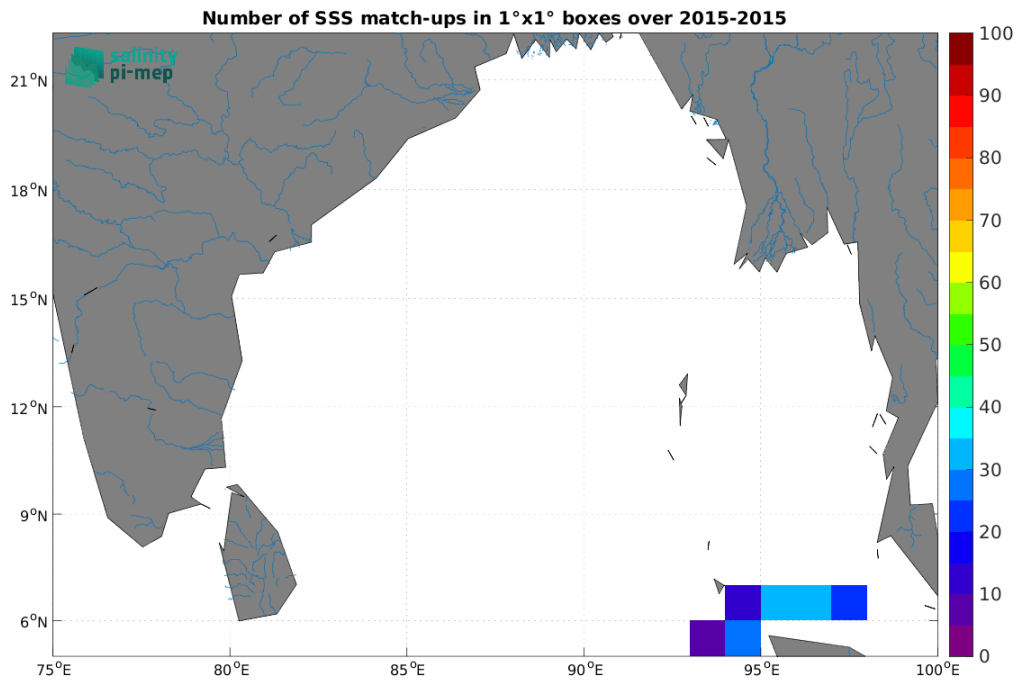
Figure 5: Number of SSS match-ups between TSG (SAMOS) SSS and the SMAP SSS L3 v5.0 - 8-Day running (JPL) SSS product for the Ganga and Brahmaputra river plumes Pi-MEP region over 1^\circ \times 1^\circ boxes and for the full satellite product period.
