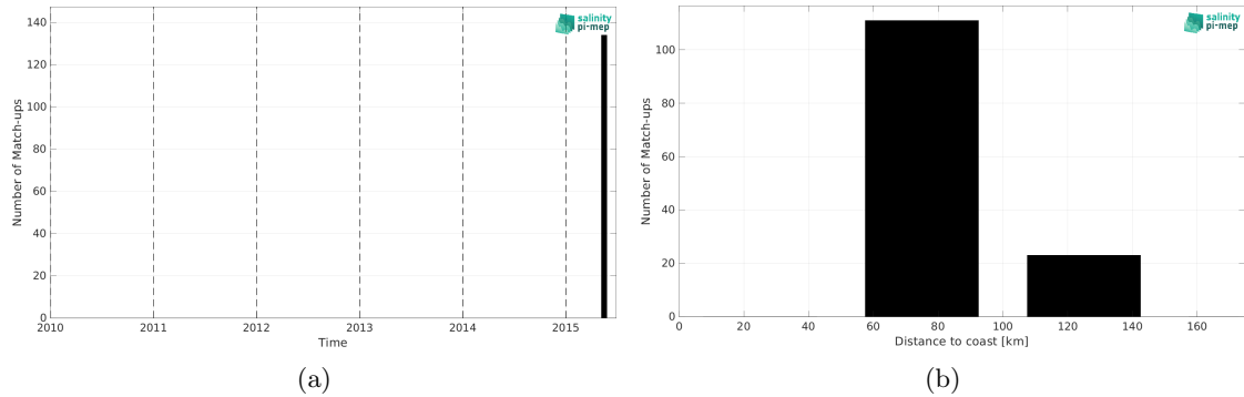
Figure 2: Number of match-ups between TSG (SAMOS) and SMAP SSS L3 v5.0 - 8-Day running (JPL) SSS as a function of time (a) and as function of the distance to coast (b) over the Ganga and Brahmaputra river plumes Pi-MEP region and for the full satellite product period.
