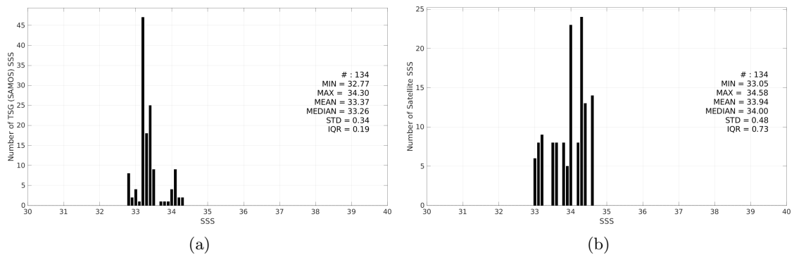
Figure 3: Histograms of SSS from TSG (SAMOS) (a) and SMAP SSS L3 v5.0 - 8-Day running (JPL) (b) considering all match-up pairs per bins of 0.1 over the Ganga and Brahmaputra river plumes Pi-MEP region and for the full satellite product period.
