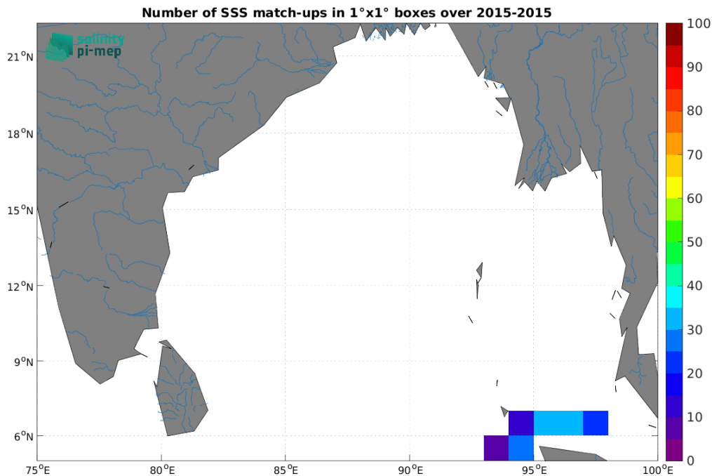
Figure 4: Number of SSS match-ups between TSG (SAMOS) SSS and the SMAP SSS L3 v5.0 - 8-Day running (JPL) SSS product for the Ganga and Brahmaputra river plumes Pi-MEP region over 1^\circ \times 1^\circ boxes and for the full satellite product period.
