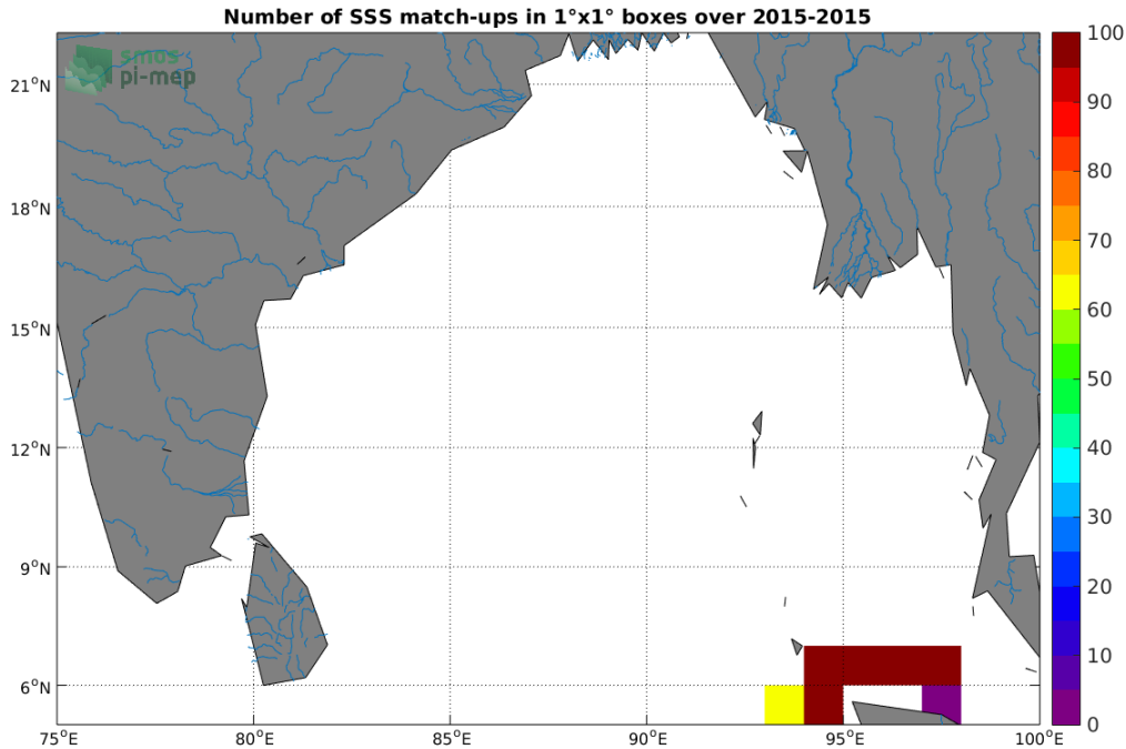
Figure 4: Number of SSS match-ups between TSG (SAMOS) SSS and the SMAP SSS L3 v5.0 - 8-Day running (JPL) SSS product for the Ganga and Brahmaputra river plumes Pi-MEP region over 1°x1° boxes and for the full satellite product period.
