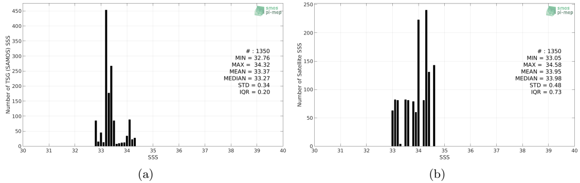
Figure 2: Histograms of SSS from TSG (SAMOS) (a) and SMAP SSS L3 v5.0 - 8-Day running (JPL) (b) considering all match-up pairs per bins of 0.1 over the Ganga and Brahmaputra river plumes Pi-MEP region and for the full satellite product period.
