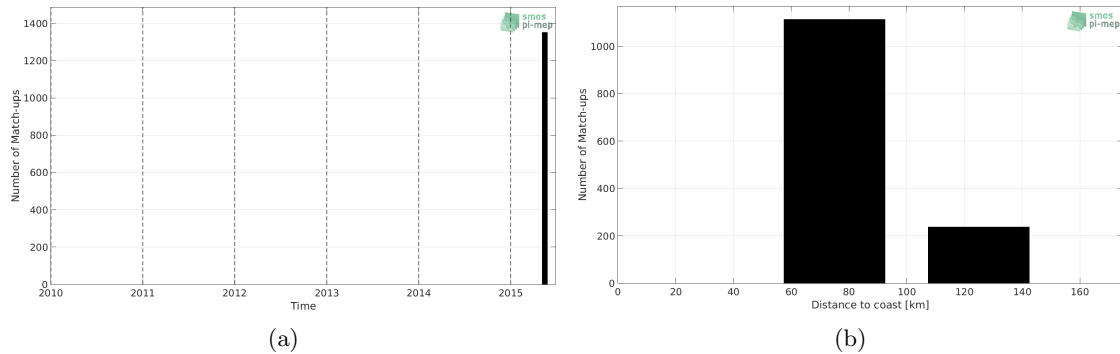
Figure 1: Number of match-ups between TSG (SAMOS) and SMAP SSS L3 v5.0 - 8-Day running (JPL) SSS as a function of time (a) and as function of the distance to coast (b) over the Ganga and Brahmaputra river plumes Pi-MEP region and for the full satellite product period.
