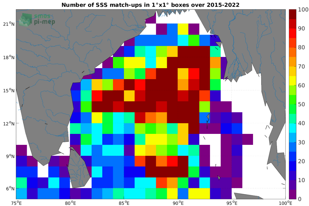
Figure 4: Number of SSS match-ups between Argo SSS and the SMAP SSS L3 v5.0 - 8-Day running (JPL) SSS product for the Ganga and Brahmaputra river plumes Pi-MEP region over 1^\circ \times 1^\circ boxes and for the full satellite product period.
