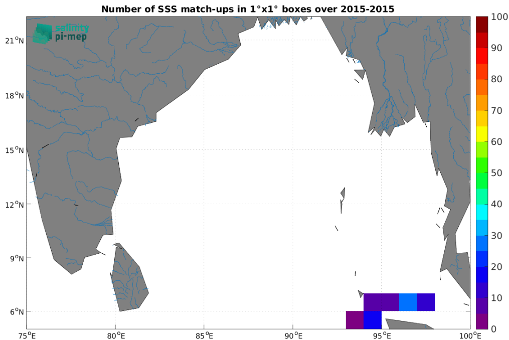
Figure 5: Number of SSS match-ups between TSG (SAMOS) SSS and the SMAP SSS L3 v5.0 - Monthly (JPL) SSS product for the Ganga and Brahmaputra river plumes Pi-MEP region over 1^\circ \times 1^\circ boxes and for the full satellite product period.
