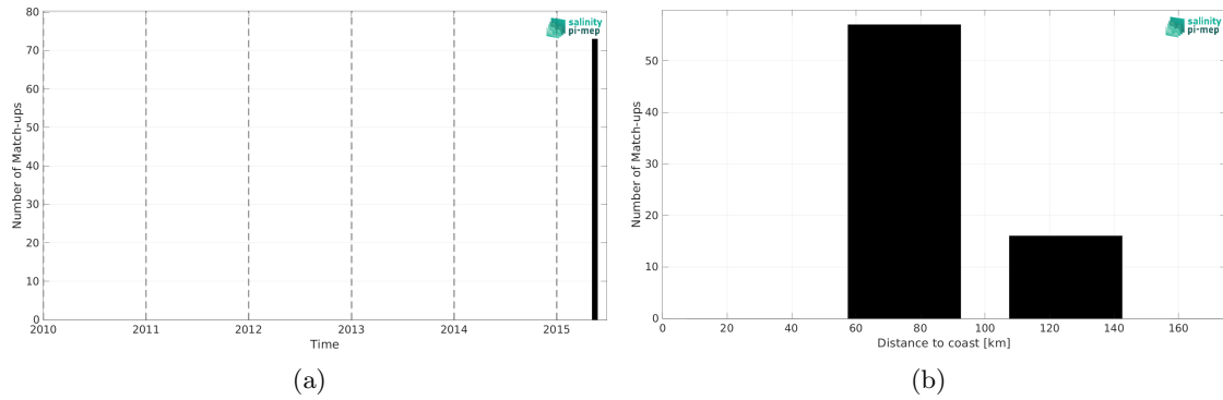
Figure 2: Number of match-ups between TSG (SAMOS) and SMAP SSS L3 v5.0 - Monthly (JPL) SSS as a function of time (a) and as function of the distance to coast (b) over the Ganga and Brahmaputra river plumes Pi-MEP region and for the full satellite product period.
