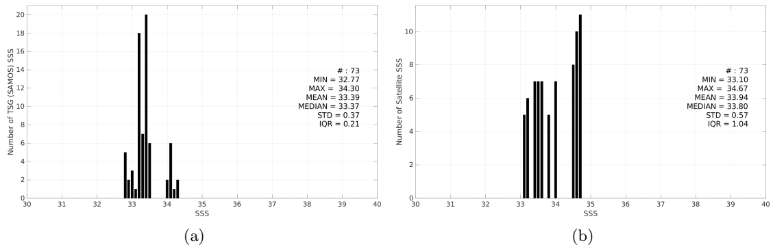
Figure 3: Histograms of SSS from TSG (SAMOS) (a) and SMAP SSS L3 v5.0 - Monthly (JPL) (b) considering all match-up pairs per bins of 0.1 over the Ganga and Brahmaputra river plumes Pi-MEP region and for the full satellite product period.
