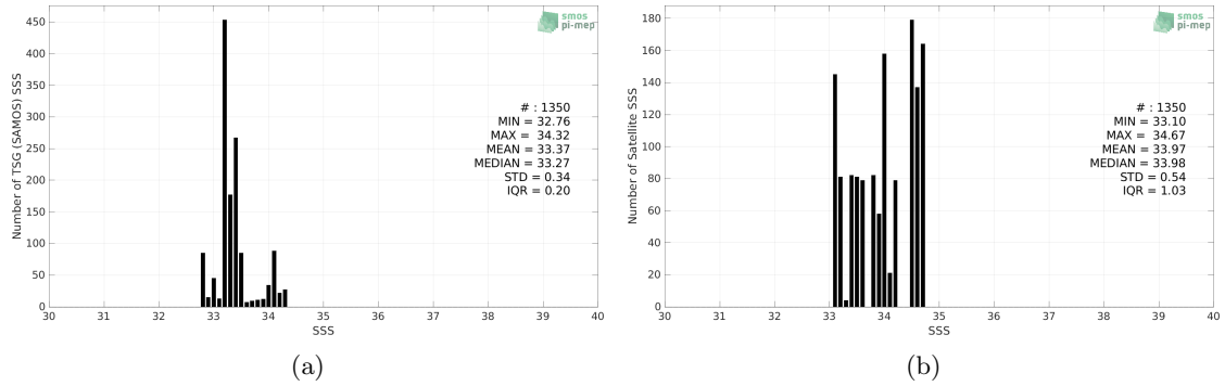
Figure 2: Histograms of SSS from TSG (SAMOS) (a) and SMAP SSS L3 v5.0 - Monthly (JPL) (b) considering all match-up pairs per bins of 0.1 over the Ganga and Brahmaputra river plumes Pi-MEP region and for the full satellite product period.
