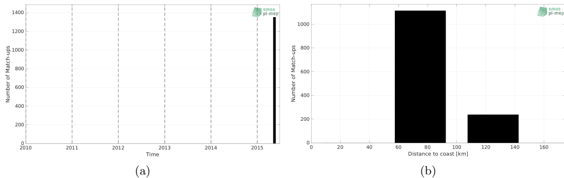
Figure 1: Number of match-ups between TSG (SAMOS) and SMAP SSS L3 v5.0 - Monthly (JPL) SSS as a function of time (a) and as function of the distance to coast (b) over the Ganga and Brahmaputra river plumes Pi-MEP region and for the full satellite product period.
