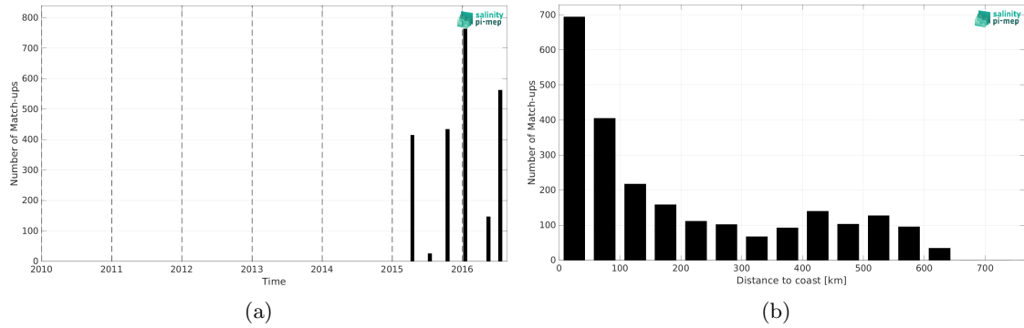
Figure 2: Number of match-ups between TSG (LEGOS-DM) and SMAP SSS L3 v5.0 - Monthly (JPL) SSS as a function of time (a) and as function of the distance to coast (b) over the Ganga and Brahmaputra river plumes Pi-MEP region and for the full satellite product period.
