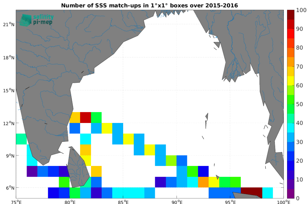
Figure 5: Number of SSS match-ups between TSG (LEGOS-DM) SSS and the SMAP SSS L3 v5.0 - Monthly (JPL) SSS product for the Ganga and Brahmaputra river plumes Pi-MEP region over 1^\circ \times 1^\circ boxes and for the full satellite product period.
