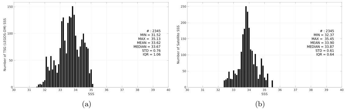
Figure 3: Histograms of SSS from TSG (LEGOS-DM) (a) and SMAP SSS L3 v5.0 - Monthly (JPL) (b) considering all match-up pairs per bins of 0.1 over the Ganga and Brahmaputra river plumes Pi-MEP region and for the full satellite product period.
