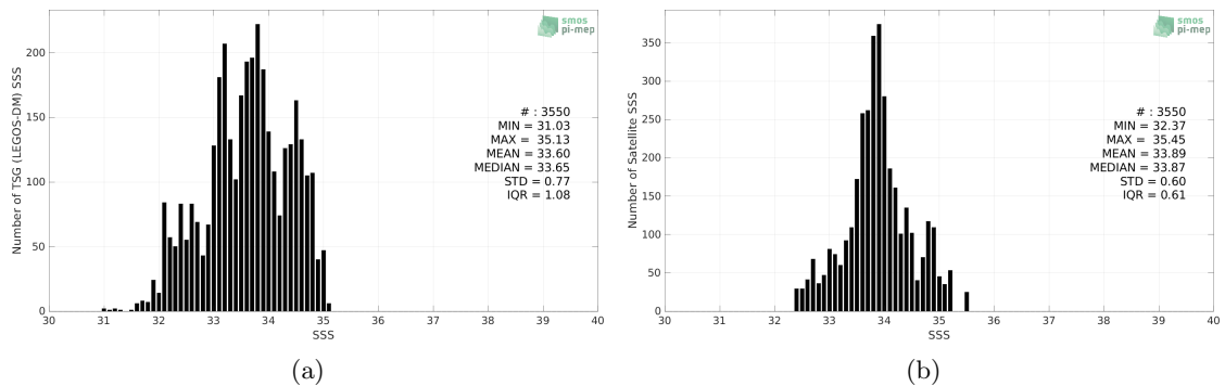
Figure 2: Histograms of SSS from TSG (LEGOS-DM) (a) and SMAP SSS L3 v5.0 - Monthly (JPL) (b) considering all match-up pairs per bins of 0.1 over the Ganga and Brahmaputra river plumes Pi-MEP region and for the full satellite product period.
