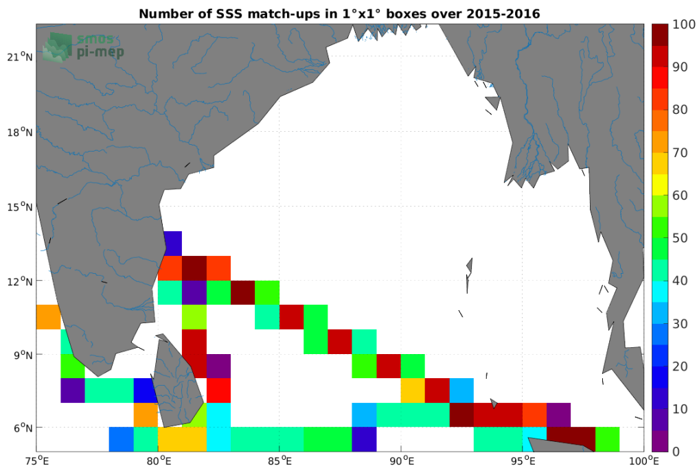
Figure 4: Number of SSS match-ups between TSG (LEGOS-DM) SSS and the SMAP SSS L3 v5.0 - Monthly (JPL) SSS product for the Ganga and Brahmaputra river plumes Pi-MEP region over 1^\circ \times 1^\circ boxes and for the full satellite product period.
