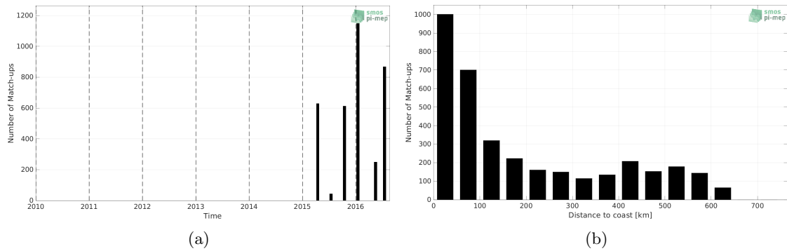
Figure 1: Number of match-ups between TSG (LEGOS-DM) and SMAP SSS L3 v5.0 - Monthly (JPL) SSS as a function of time (a) and as function of the distance to coast (b) over the Ganga and Brahmaputra river plumes Pi-MEP region and for the full satellite product period.
