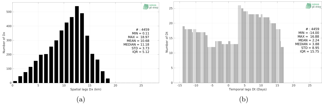
Figure 4: Histograms of the spatial (a) and temporal (b) lags between the location/time of the Surface drifters pixels measurement and the date of the corresponding SMAP SSS L3 v5.0 - Monthly (JPL) SSS pixel.
