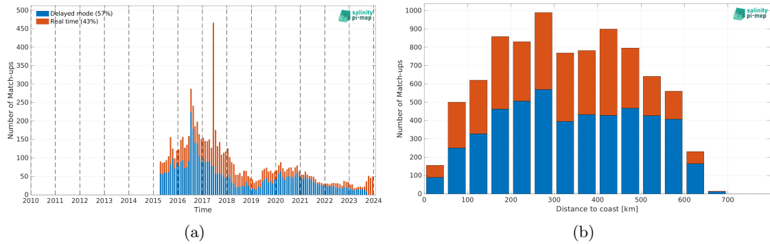
Figure 2: Number of match-ups between Argo and SMAP SSS L3 v5.0 - Monthly (JPL) SSS as a function of time (a) and as function of the distance to coast (b) over the Ganga and Brahmaputra river plumes Pi-MEP region and for the full satellite product period.
