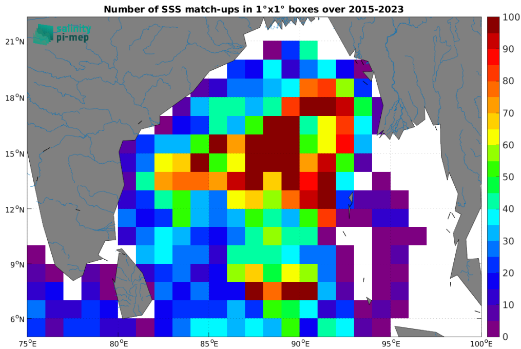
Figure 5: Number of SSS match-ups between Argo SSS and the SMAP SSS L3 v5.0 - Monthly (JPL) SSS product for the Ganga and Brahmaputra river plumes Pi-MEP region over 1^\circ \times 1^\circ boxes and for the full satellite product period.
