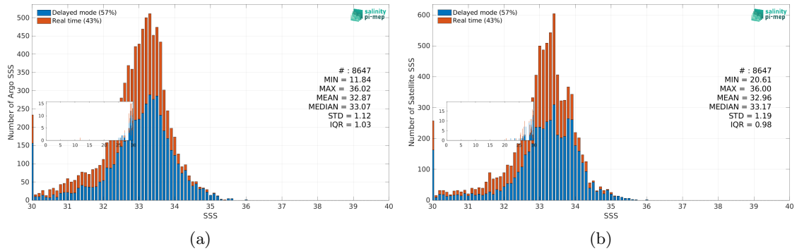
Figure 3: Histograms of SSS from Argo (a) and SMAP SSS L3 v5.0 - Monthly (JPL) (b) considering all match-up pairs per bins of 0.1 over the Ganga and Brahmaputra river plumes Pi-MEP region and for the full satellite product period.
