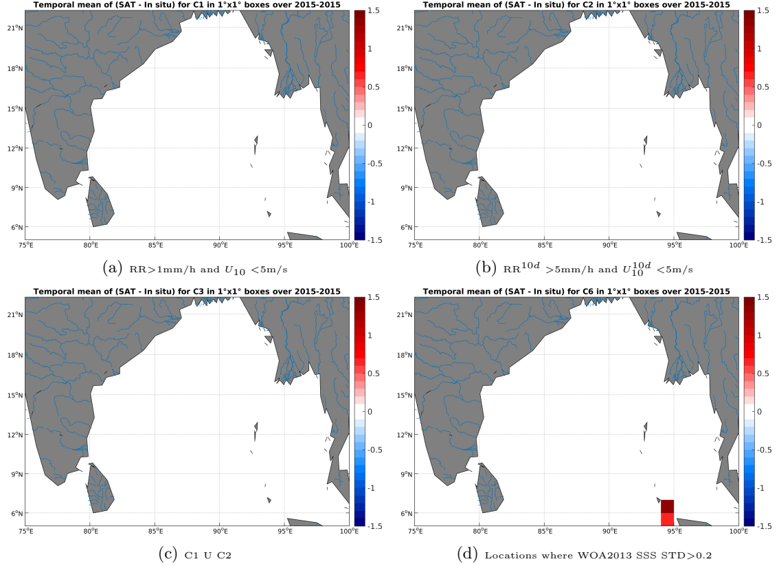
Figure 12: Temporal mean gridded over spatial boxes of size 1^\circ \times 1^\circ of \Delta SSS (SMAP-L3-JPL-V4-8DAY-RUNNING-60KM - TSG-SAMOS) for 4 different subdatasets corresponding to: RR > 1 mm/h and U_{10} < 5 m/s (a), RR^{10d} > 5 mm/h and U_{10}^{10d} < 5 m/s (b), C1 U C2 (c), Locations where WOA2013 SSS STD > 0.2 (d).
