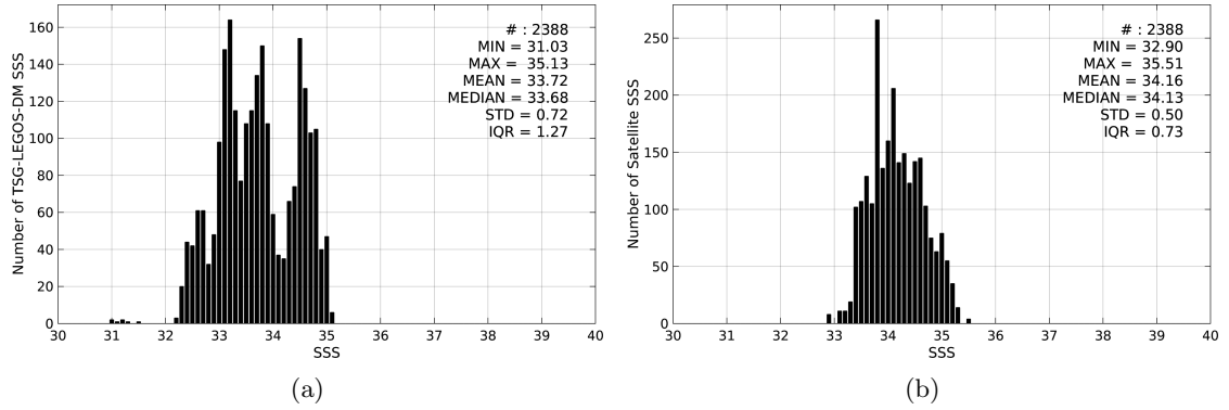
Figure 2: Histograms of SSS from TSG-LEGOS-DM (a) and SMAP-L3-JPL-V4-8DAY-RUNNING-60KM (b) considering all match-up pairs per bins of 0.1 over the Ganga and Brahmaputra river plumes Pi-MEP region and for the full satellite product period.
