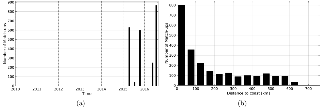
Figure 1: Number of match-ups between TSG-LEGOS-DM and SMAP-L3-JPL-V4-8DAY-RUNNING-60KM SSS as a function of time (a) and as function of the distance to coast (b) over the Ganga and Brahmaputra river plumes Pi-MEP region and for the full satellite product period.
