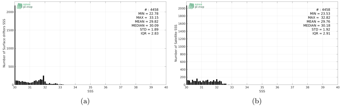
Figure 2: Histograms of SSS from Surface drifters (a) and SMAP-L3-JPL-V4-8DAY-RUNNING-60KM (b) considering all match-up pairs per bins of 0.1 over the Ganga and Brahmaputra river plumes Pi-MEP region and for the full satellite product period.
