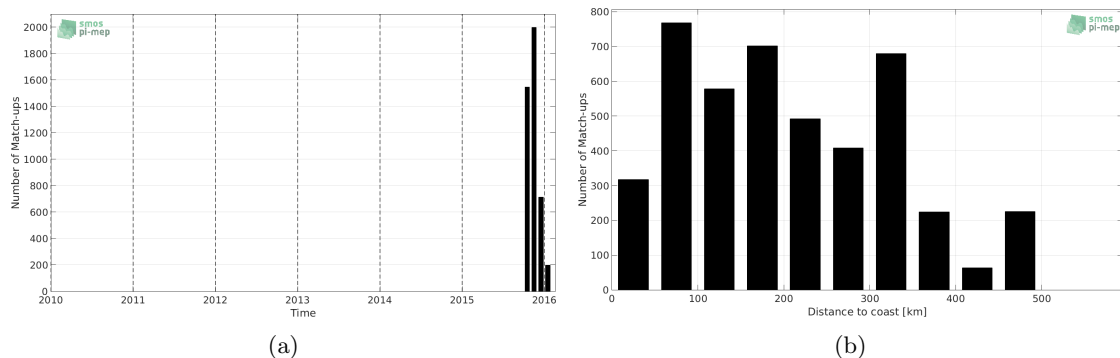
Figure 1: Number of match-ups between Surface drifters and SMAP-L3-JPL-V4-8DAY-RUNNING-60KM SSS as a function of time (a) and as function of the distance to coast (b) over the Ganga and Brahmaputra river plumes Pi-MEP region and for the full satellite product period.
