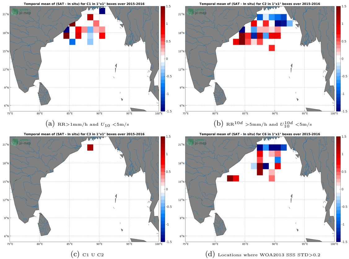
Figure 11: Temporal mean gridded over spatial boxes of size 1^\circ \times 1^\circ of \Delta SSS (SMAP-L3-JPL-V4-8DAY-RUNNING-60KM - Surface drifters) for 4 different subdatasets corresponding to: RR > 1 mm/h and U_{10} < 5 m/s (a), RR 10d > 5 mm/h and U_{10}^{10d} < 5 m/s (b), C1 U C2 (c), Locations where WOA2013 SSS STD > 0.2 (d).
