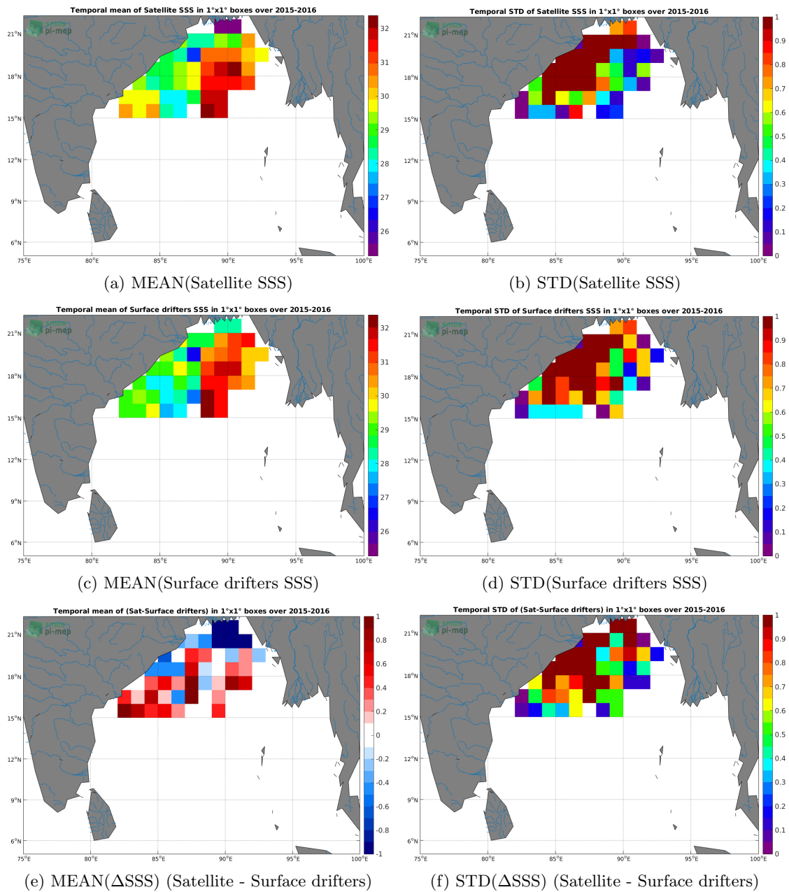
Figure 5: Temporal mean (left) and STD (right) of SSS from SMAP-L3-JPL-V4-8DAY-RUNNING-60KM (top), Surface drifters (middle), and of \Delta SSS (Satellite - Surface drifters). Only match-up pairs are used to generate these maps.
