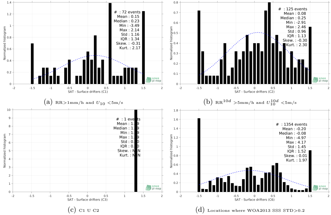
Figure 12: Normalized histogram of \Delta\text{SSS} (SMAP-L3-JPL-V4-8DAY-RUNNING-60KM - Surface drifters) for 6 different subdatasets corresponding to: RR > 1mm/h and U_{10} < 5\text{m/s} (a), RR^{10d} > 5\text{mm/h} and U_{10}^{10d} < 5\text{m/s} (b), C1 U C2 (c), Locations where WOA2013 SSS STD > 0.2 (d).
