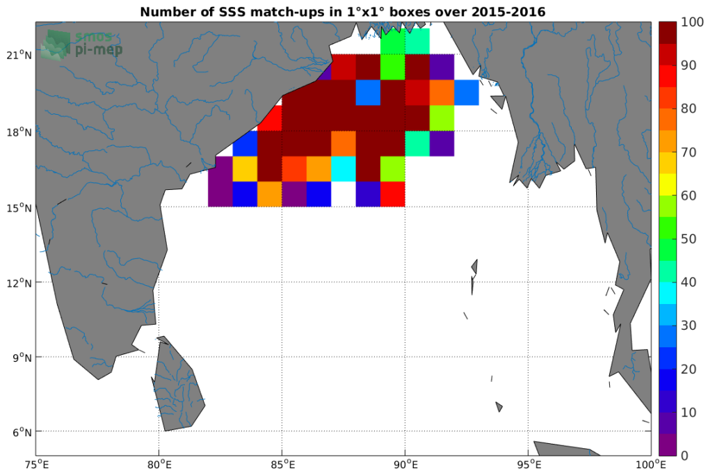
Figure 3: Number of SSS match-ups between Surface drifters SSS and the SMAP-L3-JPL-V4-8DAY-RUNNING-60KM SSS product for the Ganga and Brahmaputra river plumes Pi-MEP region over 1°x1° boxes and for the full satellite product period.
