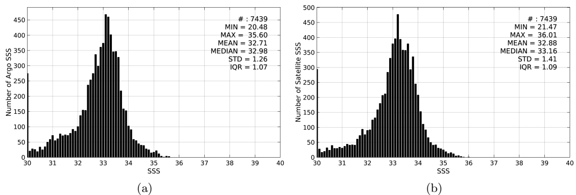
Figure 2: Histograms of SSS from Argo (a) and SMAP-L3-JPL-V4-8DAY-RUNNING-60KM (b) considering all match-up pairs per bins of 0.1 over the Ganga and Brahmaputra river plumes Pi-MEP region and for the full satellite product period.
