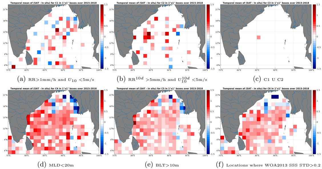
Figure 12: Temporal mean gridded over spatial boxes of size 1^\circ \times 1^\circ of \Delta SSS (SMAP-L3-JPL-V4-8DAY-RUNNING-60KM - Argo) for 6 different subdatasets corresponding to:RR>1mm/h and U_{10} < 5\text{m/s} (a), RR^{10d} > 5\text{mm/h} and U_{10}^{10d} < 5\text{m/s} (b), C1 U C2 (c),MLD<20m (d),BLT>10m (e),Locations where WOA2013 SSS STD>0.2 (f).
