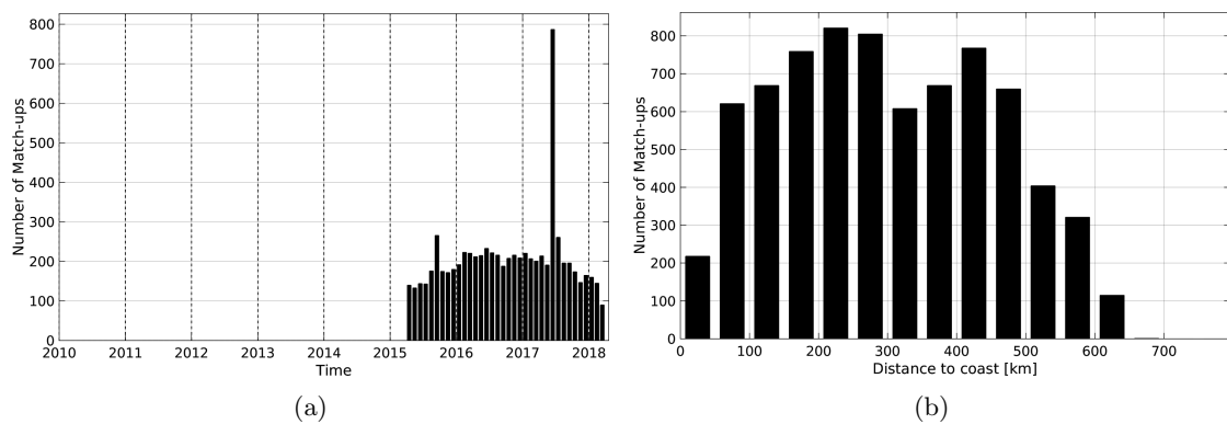
Figure 1: Number of match-ups between Argo and SMAP-L3-JPL-V4-8DAY-RUNNING-60KM SSS as a function of time (a) and as function of the distance to coast (b) over the Ganga and Brahmaputra river plumes Pi-MEP region and for the full satellite product period.
