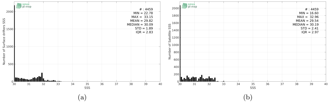
Figure 2: Histograms of SSS from Surface drifters (a) and SMAP-L3-JPL-V4-MONTHLY-60KM (b) considering all match-up pairs per bins of 0.1 over the Ganga and Brahmaputra river plumes Pi-MEP region and for the full satellite product period.
