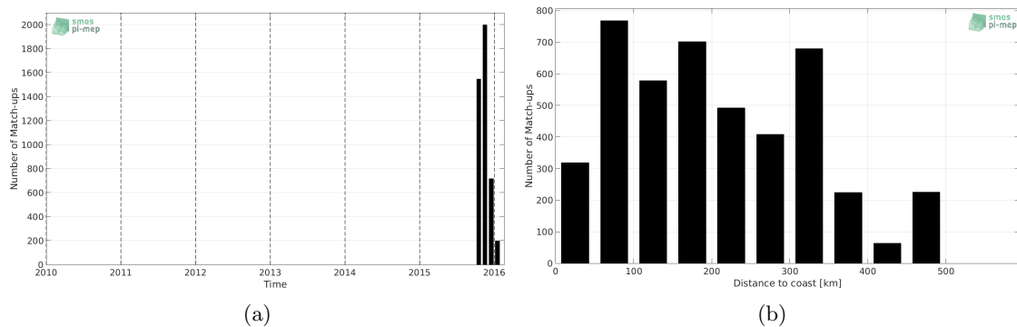
Figure 1: Number of match-ups between Surface drifters and SMAP-L3-JPL-V4-MONTHLY-60KM SSS as a function of time (a) and as function of the distance to coast (b) over the Ganga and Brahmaputra river plumes Pi-MEP region and for the full satellite product period.
