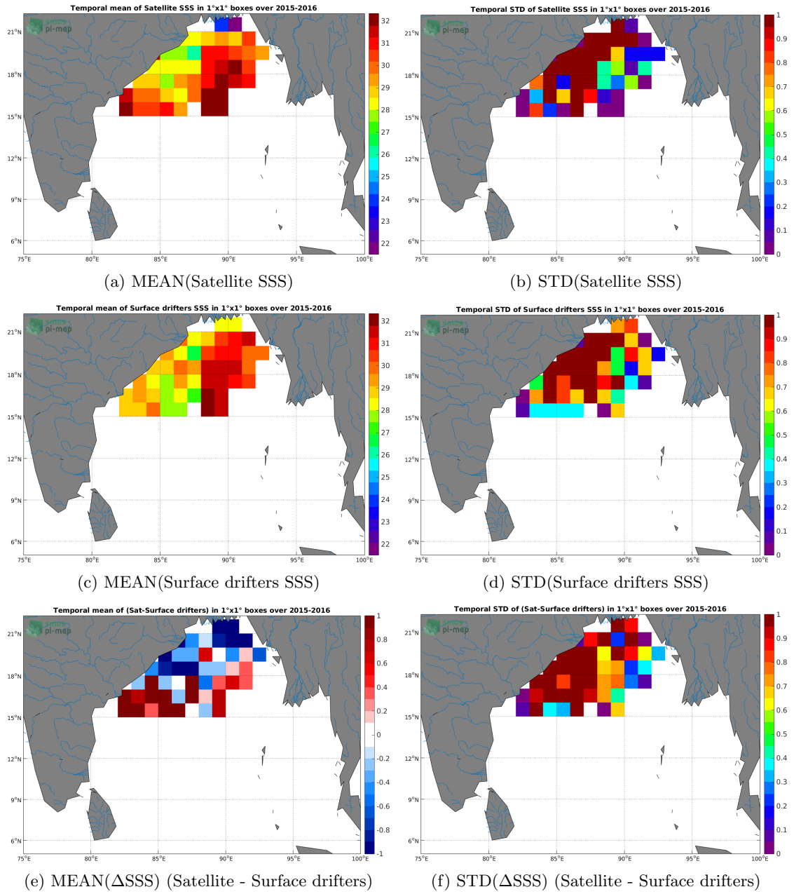
Figure 5: Temporal mean (left) and STD (right) of SSS from SMAP-L3-JPL-V4-MONTHLY-60KM (top), Surface drifters (middle), and of \Delta SSS (Satellite - Surface drifters). Only match-up pairs are used to generate these maps.
