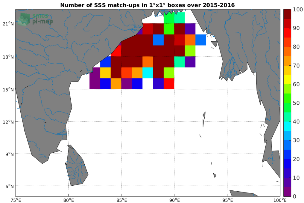
Figure 3: Number of SSS match-ups between Surface drifters SSS and the SMAP-L3-JPL-V4-MONTHLY-60KM SSS product for the Ganga and Brahmaputra river plumes Pi-MEP region over 1°x1° boxes and for the full satellite product period.
