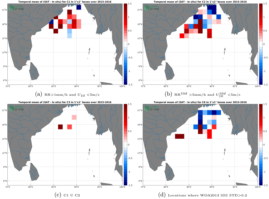
Figure 11: Temporal mean gridded over spatial boxes of size 1^\circ \times 1^\circ of \Delta SSS (SMAP-L3-JPL-V4-MONTHLY-60KM - Surface drifters) for 4 different subdatasets corresponding to: RR > 1mm/h and U_{10} < 5\text{m/s} (a), RR^{10d} > 5\text{mm/h} and U_{10}^{10d} < 5\text{m/s} (b), C1 U C2 (c), Locations where WOA2013 SSS STD > 0.2 (d).
