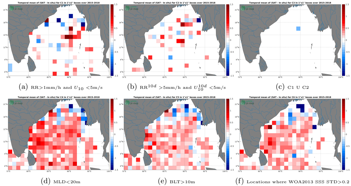
Figure 12: Temporal mean gridded over spatial boxes of size 1^\circ \times 1^\circ of \Delta SSS (SMAP-L3-JPL-V4-MONTHLY-60KM - Argo) for 6 different subdatasets corresponding to: RR > 1\text{mm/h} and U_{10} < 5\text{m/s} (a), RR^{10d} > 5\text{mm/h} and U_{10}^{10d} < 5\text{m/s} (b), C1 U C2 (c), MLD < 20\text{m} (d), BLT > 10\text{m} (e), Locations where WOA2013 SSS STD > 0.2 (f).
