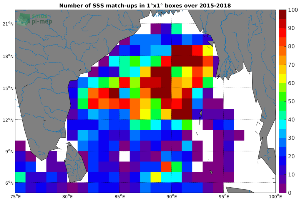
Figure 4: Number of SSS match-ups between Argo SSS and the SMAP-L3-JPL-V4-MONTHLY-60KM SSS product for the Ganga and Brahmaputra river plumes Pi-MEP region over 1°x1° boxes and for the full satellite product period.
