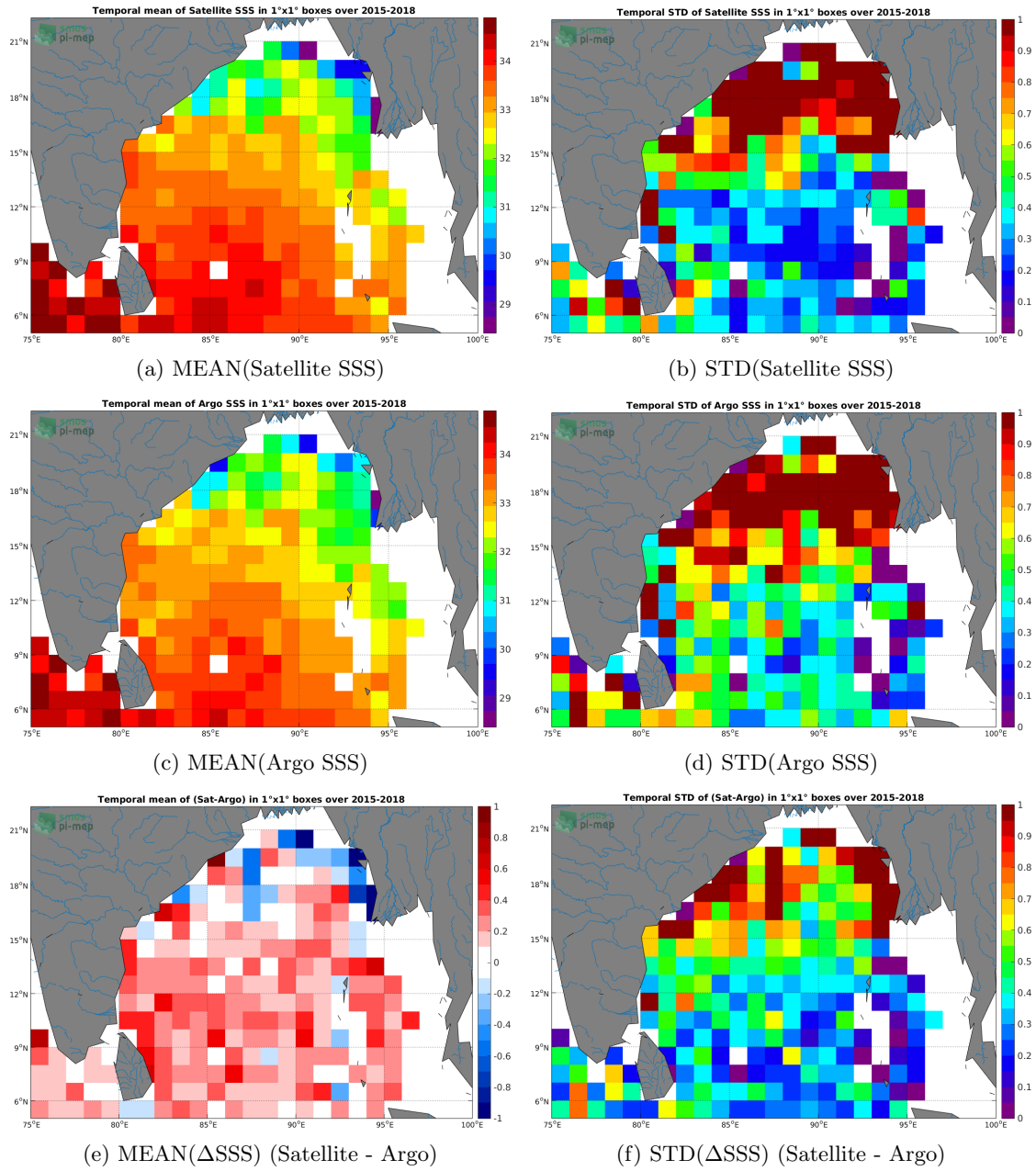
Figure 6: Temporal mean (left) and STD (right) of SSS from SMAP-L3-JPL-V4-MONTHLY-60KM (top), Argo (middle), and of \Delta SSS (Satellite - Argo). Only match-up pairs are used to generate these maps.
