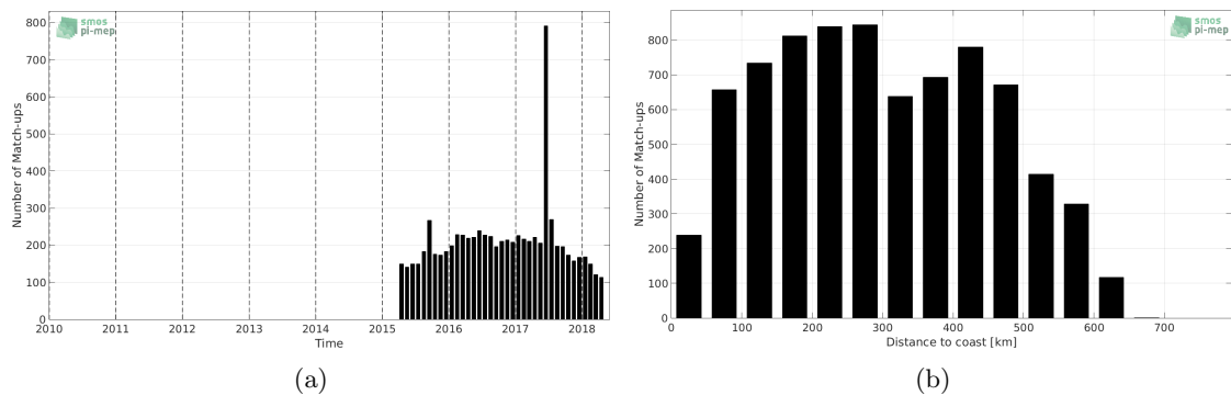
Figure 1: Number of match-ups between Argo and SMAP-L3-JPL-V4-MONTHLY-60KM SSS as a function of time (a) and as function of the distance to coast (b) over the Ganga and Brahmaputra river plumes Pi-MEP region and for the full satellite product period.
