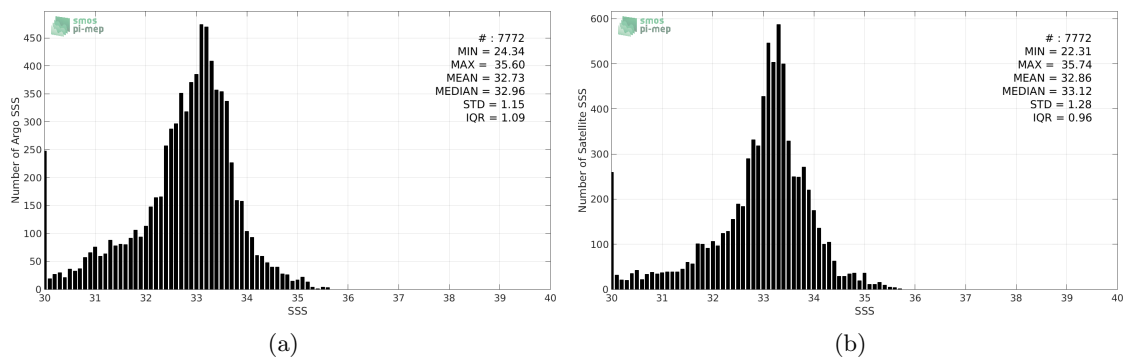
Figure 2: Histograms of SSS from Argo (a) and SMAP-L3-JPL-V4-MONTHLY-60KM (b) considering all match-up pairs per bins of 0.1 over the Ganga and Brahmaputra river plumes Pi-MEP region and for the full satellite product period.
