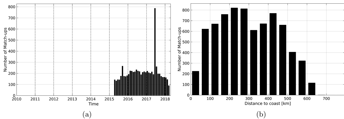
Figure 1: Number of match-ups between Argo and SMAP-L3-JPL-V4-MONTHLY-60KM SSS as a function of time (a) and as function of the distance to coast (b) over the Ganga and Brahmaputra river plumes Pi-MEP region and for the full satellite product period.
