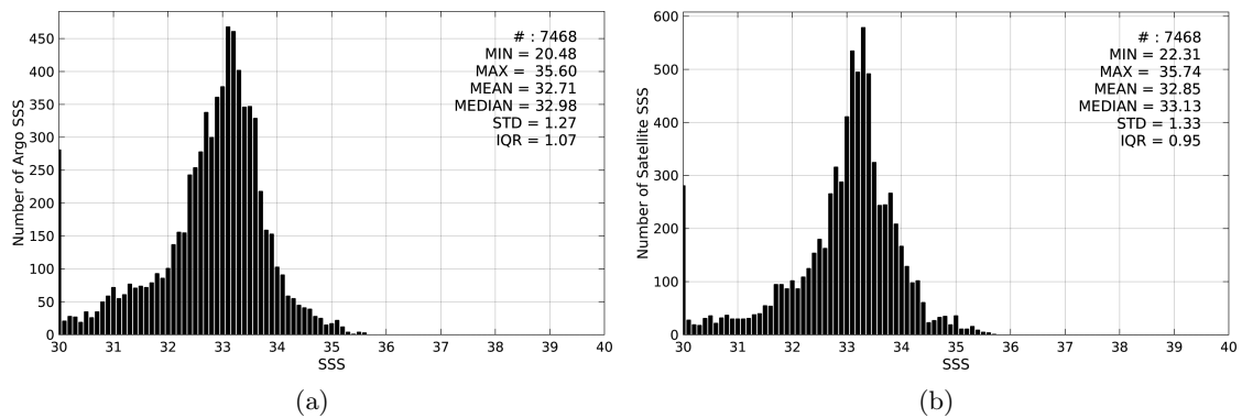
Figure 2: Histograms of SSS from Argo (a) and SMAP-L3-JPL-V4-MONTHLY-60KM (b) considering all match-up pairs per bins of 0.1 over the Ganga and Brahmaputra river plumes Pi-MEP region and for the full satellite product period.
