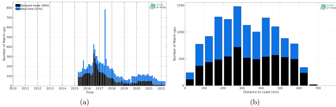
Figure 1: Number of match-ups between Argo and SMAP SSS L2-AVERAGED v5.0 (JPL) SSS as a function of time (a) and as function of the distance to coast (b) over the Ganga and Brahmaputra river plumes Pi-MEP region and for the full satellite product period.
