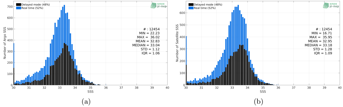
Figure 2: Histograms of SSS from Argo (a) and SMAP SSS L2-AVERAGED v5.0 (JPL) (b) considering all match-up pairs per bins of 0.1 over the Ganga and Brahmaputra river plumes Pi-MEP region and for the full satellite product period.
