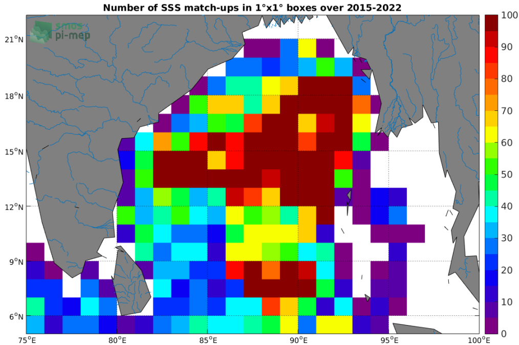
Figure 4: Number of SSS match-ups between Argo SSS and the SMAP SSS L2-AVERAGED v5.0 (JPL) SSS product for the Ganga and Brahmaputra river plumes Pi-MEP region over 1^\circ \times 1^\circ boxes and for the full satellite product period.
