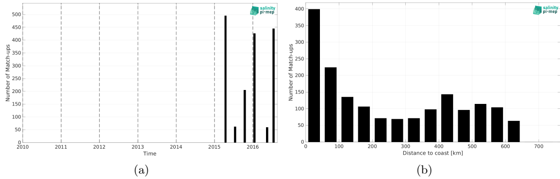
Figure 2: Number of match-ups between TSG (LEGOS-DM) and SMAP SSS L2 v6 (RSS) SSS as a function of time (a) and as function of the distance to coast (b) over the Ganga and Brahmaputra river plumes Pi-MEP region and for the full satellite product period.
