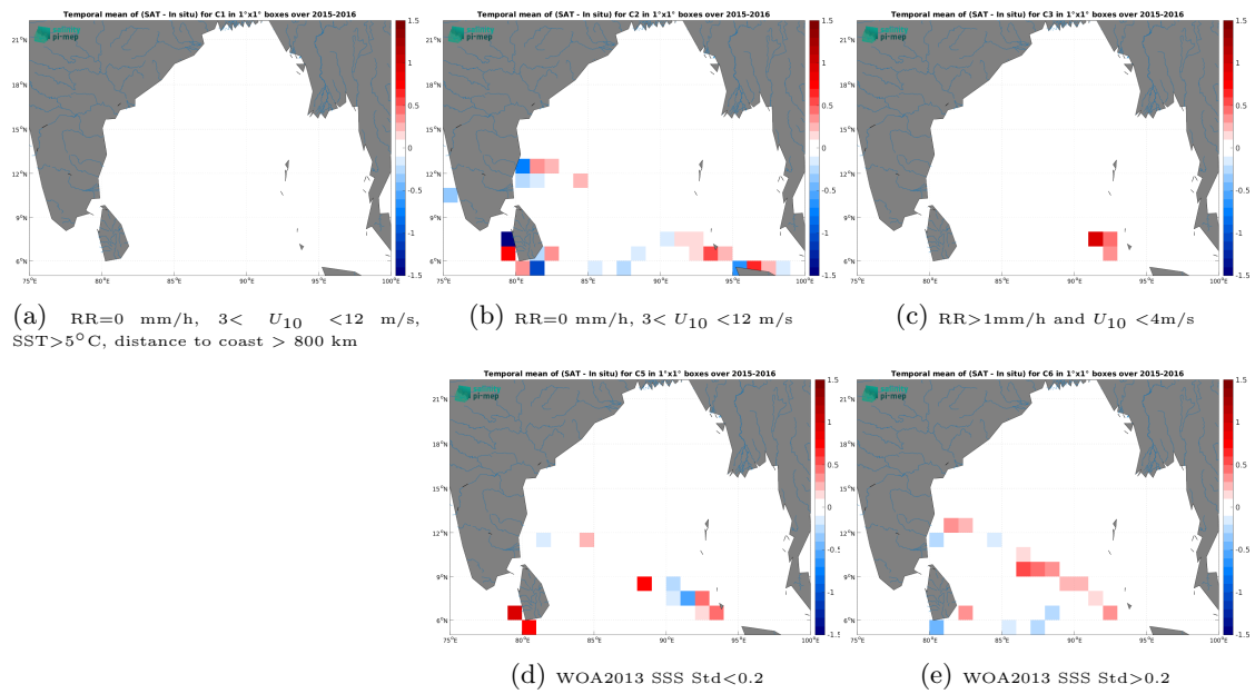
Figure 14: Temporal mean gridded over spatial boxes of size 1^\circ \times 1^\circ of \Delta SSS (SMAP SSS L2 v6 (RSS) - TSG (LEGOS-DM)) for 5 different subdatasets corresponding to:RR=0 mm/h, 3 < U_{10} < 12 m/s, SST > 5°C, distance to coast > 800 km (a), RR=0 mm/h, 3 < U_{10} < 12 m/s (b), RR > 1mm/h and U_{10} < 4 m/s (c), WOA2013 SSS Std < 0.2 (d), WOA2013 SSS Std > 0.2 (e).
