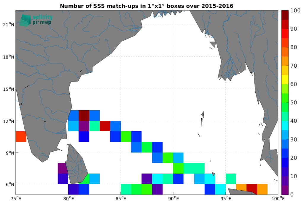
Figure 5: Number of SSS match-ups between TSG (LEGOS-DM) SSS and the SMAP SSS L2 v6 (RSS) SSS product for the Ganga and Brahmaputra river plumes Pi-MEP region over 1^\circ \times 1^\circ boxes and for the full satellite product period.
