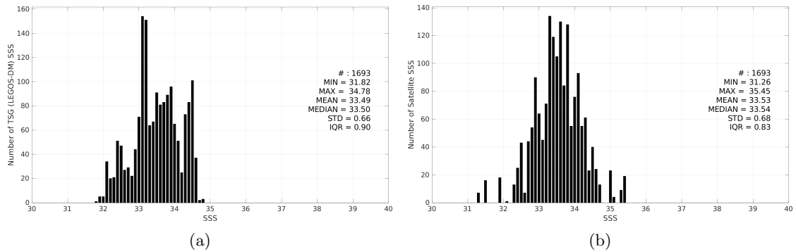
Figure 3: Histograms of SSS from TSG (LEGOS-DM) (a) and SMAP SSS L2 v6 (RSS) (b) considering all match-up pairs per bins of 0.1 over the Ganga and Brahmaputra river plumes Pi-MEP region and for the full satellite product period.
