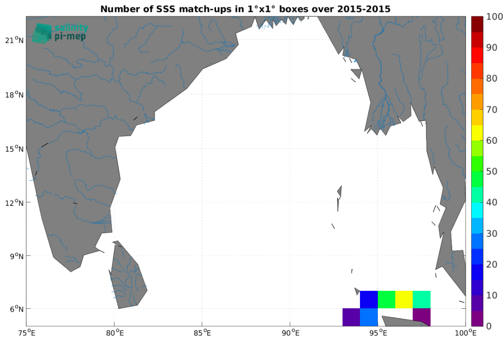
Figure 5: Number of SSS match-ups between TSG (SAMOS) SSS and the SMAP SSS L2 v6 - 40 km (RSS) SSS product for the Ganga and Brahmaputra river plumes Pi-MEP region over 1^\circ \times 1^\circ boxes and for the full satellite product period.
