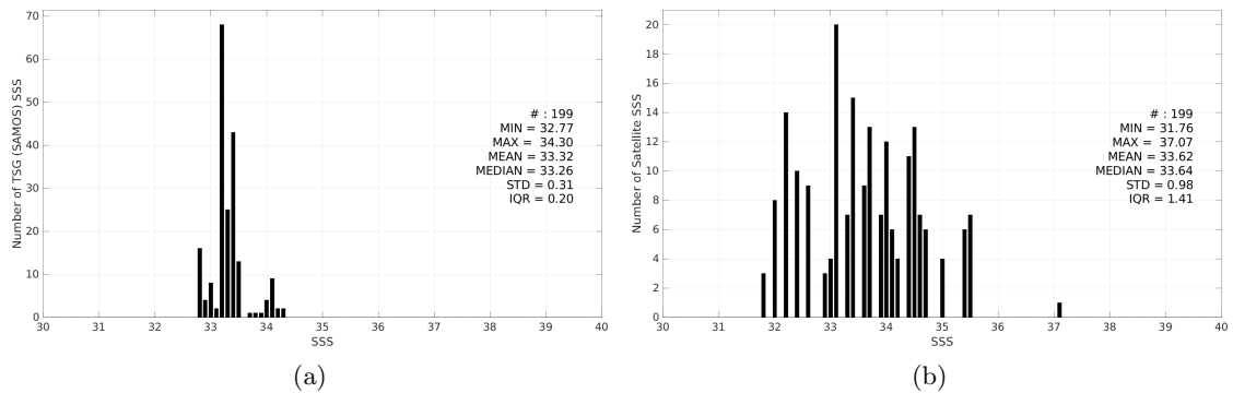
Figure 3: Histograms of SSS from TSG (SAMOS) (a) and SMAP SSS L2 v6 - 40 km (RSS) (b) considering all match-up pairs per bins of 0.1 over the Ganga and Brahmaputra river plumes Pi-MEP region and for the full satellite product period.
