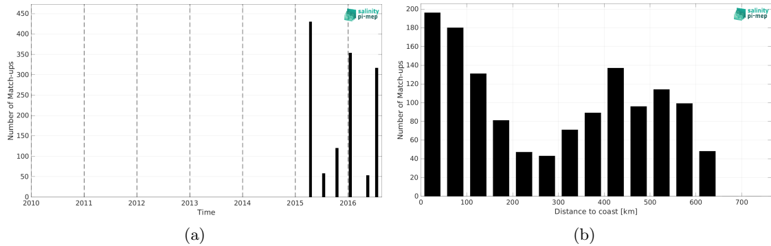
Figure 2: Number of match-ups between TSG (LEGOS-DM) and SMAP SSS L2 v6 - 40 km (RSS) SSS as a function of time (a) and as function of the distance to coast (b) over the Ganga and Brahmaputra river plumes Pi-MEP region and for the full satellite product period.
