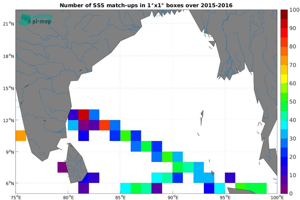
Figure 5: Number of SSS match-ups between TSG (LEGOS-DM) SSS and the SMAP SSS L2 v6 - 40 km (RSS) SSS product for the Ganga and Brahmaputra river plumes Pi-MEP region over 1^\circ \times 1^\circ boxes and for the full satellite product period.
