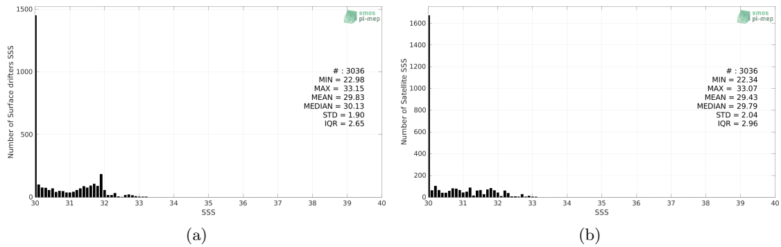
Figure 2: Histograms of SSS from Surface drifters (a) and SMAP SSS L2 v5 (RSS) (b) considering all match-up pairs per bins of 0.1 over the Ganga and Brahmaputra river plumes Pi-MEP region and for the full satellite product period.
