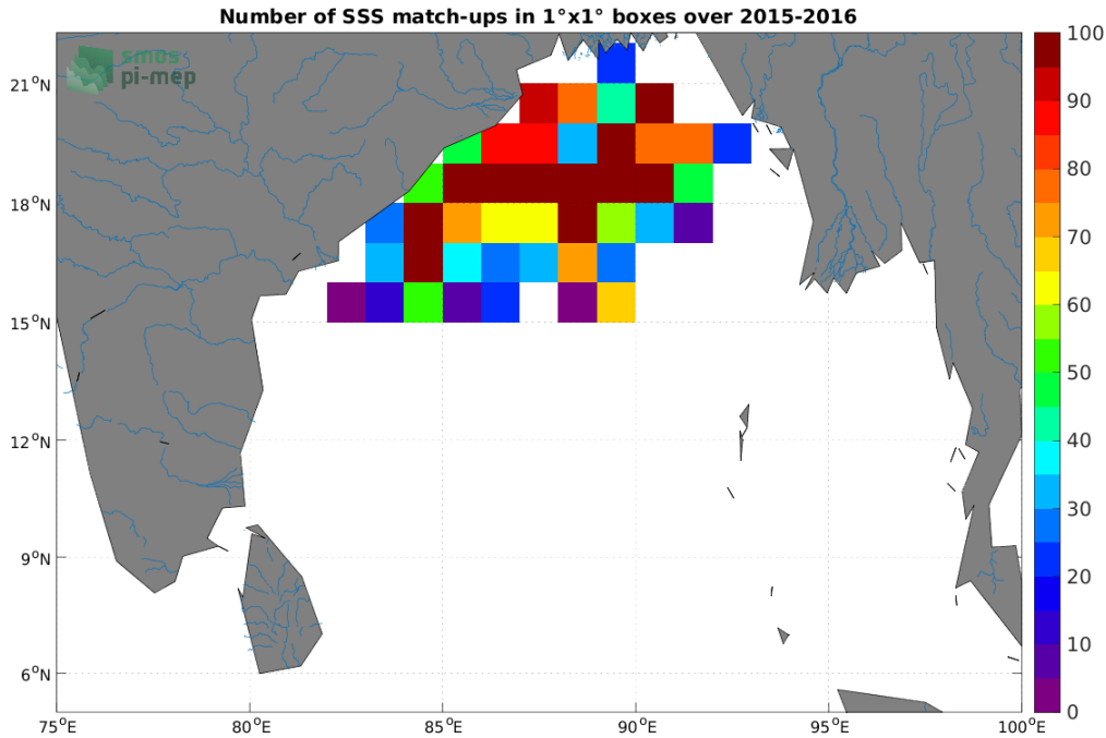
Figure 3: Number of SSS match-ups between Surface drifters SSS and the SMAP SSS L2 v5 (RSS) SSS product for the Ganga and Brahmaputra river plumes Pi-MEP region over 1°x1° boxes and for the full satellite product period.
