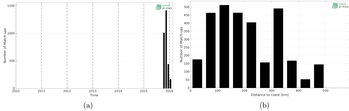
Figure 1: Number of match-ups between Surface drifters and SMAP SSS L2 v5 (RSS) SSS as a function of time (a) and as function of the distance to coast (b) over the Ganga and Brahmaputra river plumes Pi-MEP region and for the full satellite product period.
