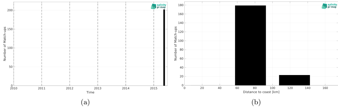
Figure 2: Number of match-ups between TSG (SAMOS) and SMAP SSS L2 v5.3 (RSS) SSS as a function of time (a) and as function of the distance to coast (b) over the Ganga and Brahmaputra river plumes Pi-MEP region and for the full satellite product period.
