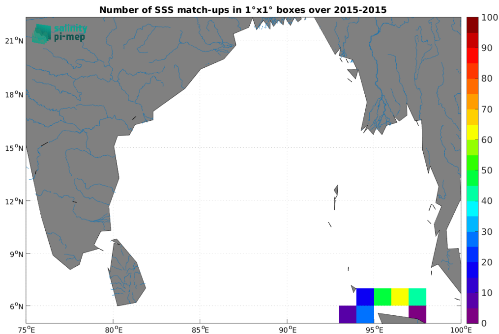
Figure 5: Number of SSS match-ups between TSG (SAMOS) SSS and the SMAP SSS L2 v5.3 (RSS) SSS product for the Ganga and Brahmaputra river plumes Pi-MEP region over 1^\circ \times 1^\circ boxes and for the full satellite product period.
