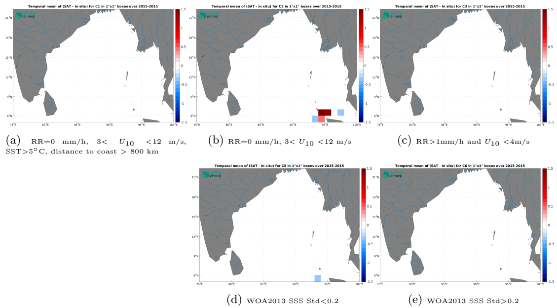
Figure 14: Temporal mean gridded over spatial boxes of size 1^\circ \times 1^\circ of \Delta SSS (SMAP SSS L2 v5.3 (RSS) - TSG (SAMOS)) for 5 different subdatasets corresponding to:RR=0 mm/h, 3 < U_{10} < 12 m/s, SST>5°C, distance to coast > 800 km (a), RR=0 mm/h, 3 < U_{10} < 12 m/s (b), RR>1mm/h and U_{10} < 4 m/s (c), WOA2013 SSS Std<0.2 (d), WOA2013 SSS Std>0.2 (e).
