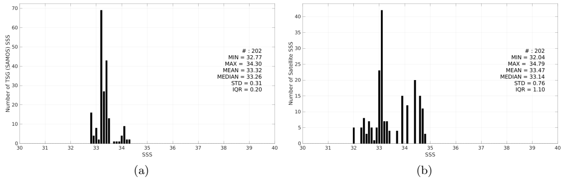
Figure 3: Histograms of SSS from TSG (SAMOS) (a) and SMAP SSS L2 v5.3 (RSS) (b) considering all match-up pairs per bins of 0.1 over the Ganga and Brahmaputra river plumes Pi-MEP region and for the full satellite product period.
