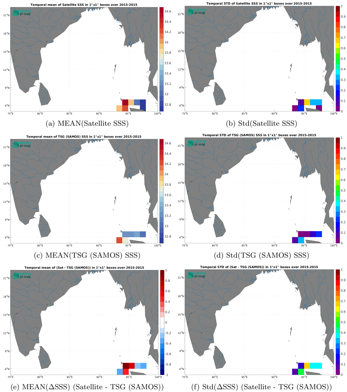
Figure 7: Temporal mean (left) and Std (right) of SSS from SMAP SSS L2 v5.3 (RSS) (top), TSG (SAMOS) (middle), and of \Delta SSS (Satellite - TSG (SAMOS)). Only match-up pairs are used to generate these maps.
