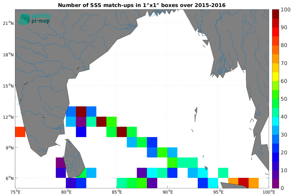
Figure 5: Number of SSS match-ups between TSG (LEGOS-DM) SSS and the SMAP SSS L2 v5.3 (RSS) SSS product for the Ganga and Brahmaputra river plumes Pi-MEP region over 1°x1° boxes and for the full satellite product period.
