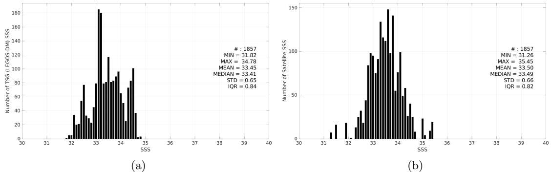
Figure 3: Histograms of SSS from TSG (LEGOS-DM) (a) and SMAP SSS L2 v5.3 (RSS) (b) considering all match-up pairs per bins of 0.1 over the Ganga and Brahmaputra river plumes Pi-MEP region and for the full satellite product period.
