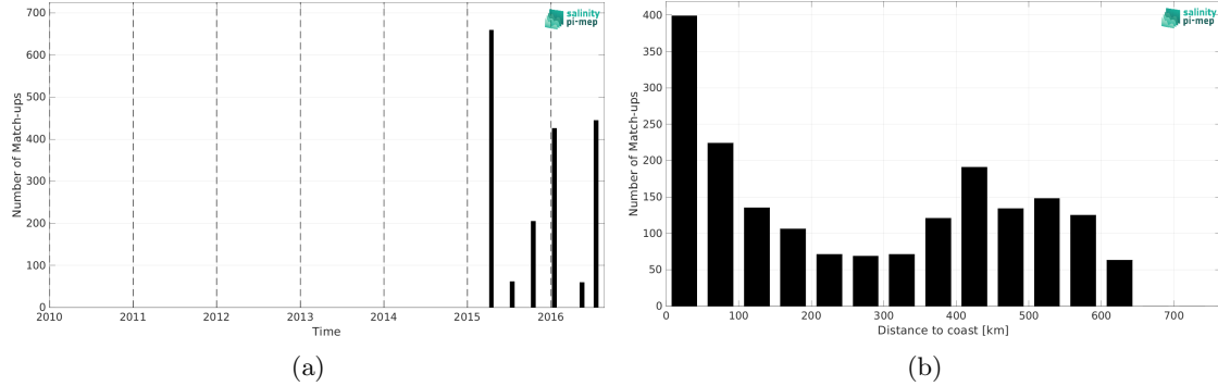
Figure 2: Number of match-ups between TSG (LEGOS-DM) and SMAP SSS L2 v5.3 (RSS) SSS as a function of time (a) and as function of the distance to coast (b) over the Ganga and Brahmaputra river plumes Pi-MEP region and for the full satellite product period.
