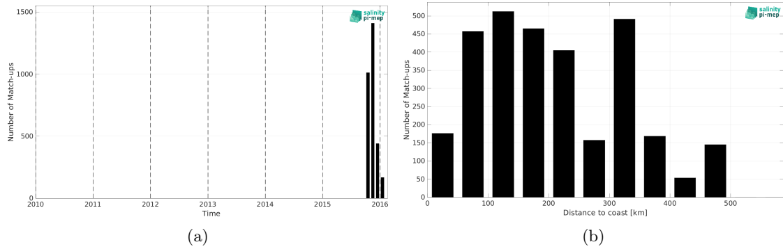
Figure 2: Number of match-ups between Surface drifters and SMAP SSS L2 v5.3 (RSS) SSS as a function of time (a) and as function of the distance to coast (b) over the Ganga and Brahmaputra river plumes Pi-MEP region and for the full satellite product period.
