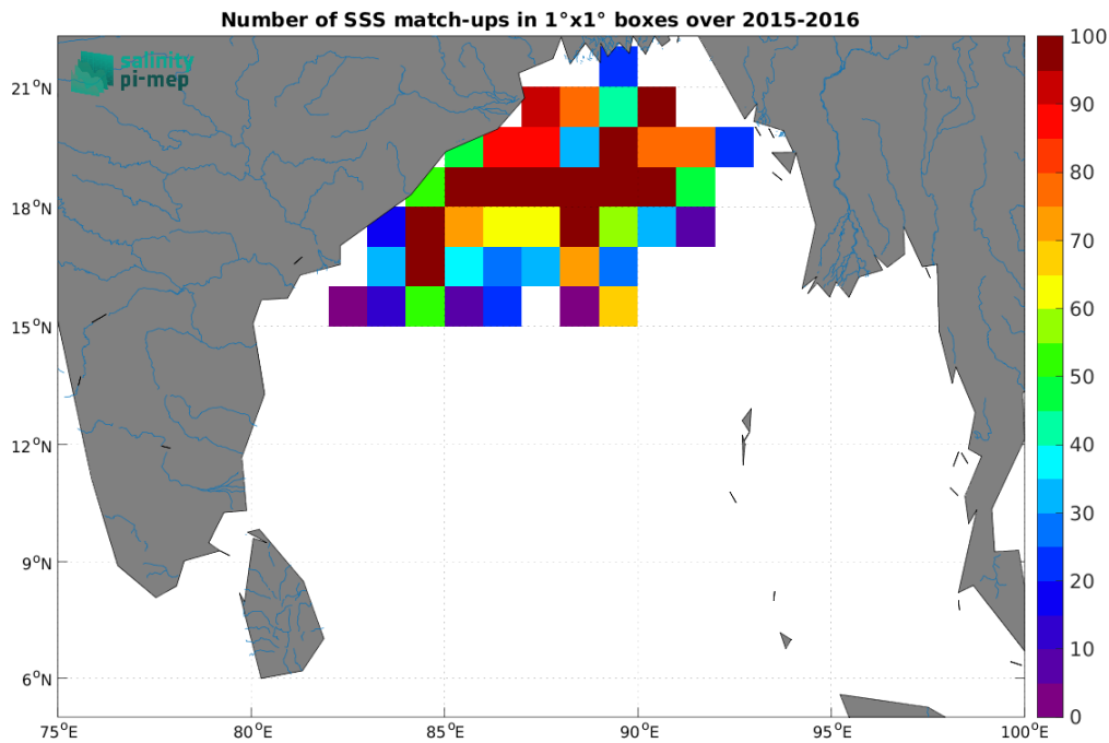
Figure 4: Number of SSS match-ups between Surface drifters SSS and the SMAP SSS L2 v5.3 (RSS) SSS product for the Ganga and Brahmaputra river plumes Pi-MEP region over 1^\circ \times 1^\circ boxes and for the full satellite product period.
