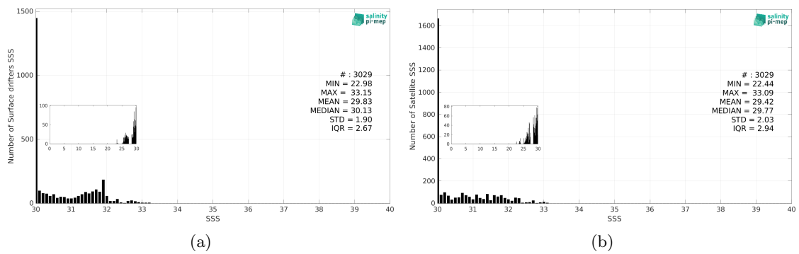
Figure 3: Histograms of SSS from Surface drifters (a) and SMAP SSS L2 v5.3 (RSS) (b) considering all match-up pairs per bins of 0.1 over the Ganga and Brahmaputra river plumes Pi-MEP region and for the full satellite product period.
