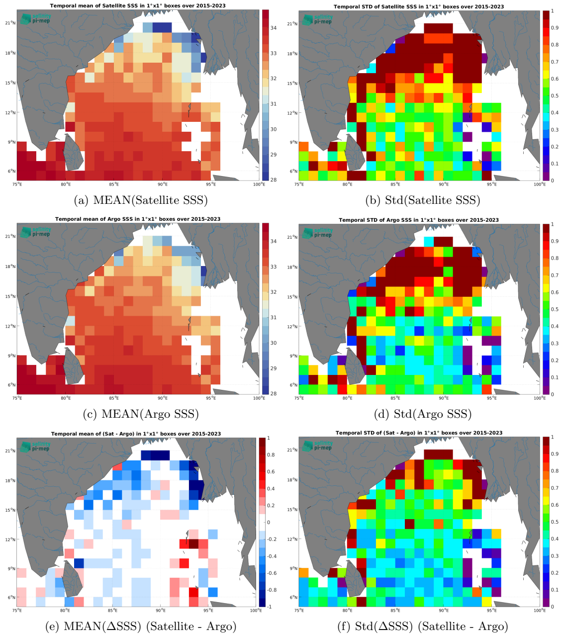
Figure 7: Temporal mean (left) and Std (right) of SSS from SMAP SSS L2 v5.3 (RSS) (top), Argo (middle), and of \Delta SSS (Satellite - Argo). Only match-up pairs are used to generate these maps.
