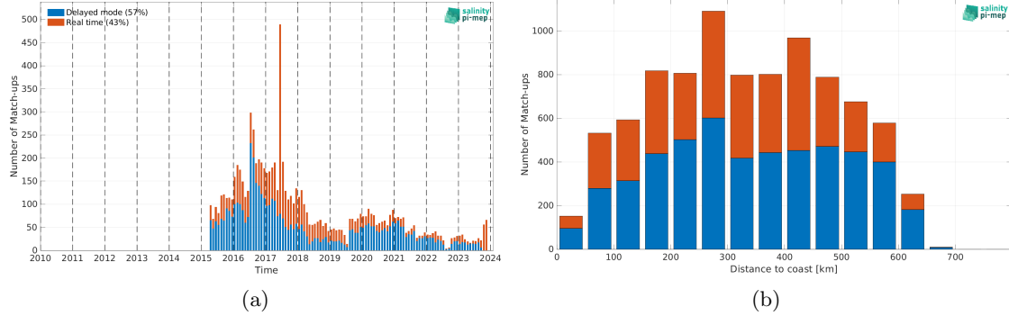
Figure 2: Number of match-ups between Argo and SMAP SSS L2 v5.3 (RSS) SSS as a function of time (a) and as function of the distance to coast (b) over the Ganga and Brahmaputra river plumes Pi-MEP region and for the full satellite product period.
