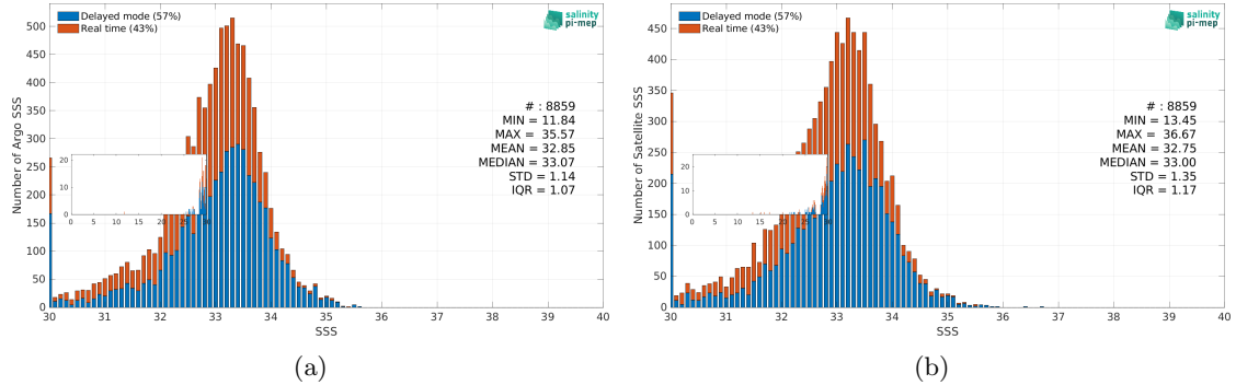
Figure 3: Histograms of SSS from Argo (a) and SMAP SSS L2 v5.3 (RSS) (b) considering all match-up pairs per bins of 0.1 over the Ganga and Brahmaputra river plumes Pi-MEP region and for the full satellite product period.
