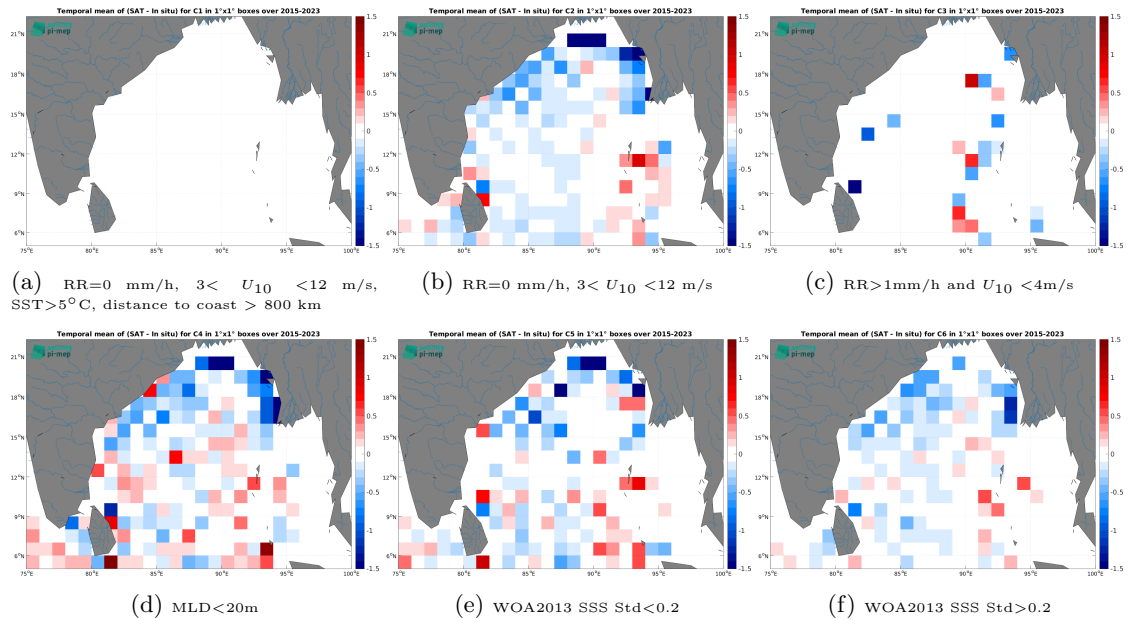
Figure 14: Temporal mean gridded over spatial boxes of size 1^\circ \times 1^\circ of \Delta SSS (SMAP SSS L2 v5.3 (RSS) - Argo) for 6 different subdatasets corresponding to:RR=0 mm/h, 3 < U_{10} < 12 m/s, SST > 5°C, distance to coast > 800 km (a), RR=0 mm/h, 3 < U_{10} < 12 m/s (b), RR > 1mm/h and U_{10} < 4 m/s (c),MLD < 20m (d),WOA2013 SSS Std < 0.2 (e),WOA2013 SSS Std > 0.2 (f).
