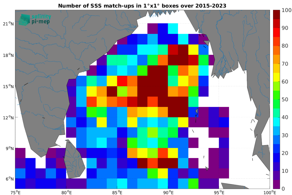
Figure 5: Number of SSS match-ups between Argo SSS and the SMAP SSS L2 v5.3 (RSS) SSS product for the Ganga and Brahmaputra river plumes Pi-MEP region over 1^\circ \times 1^\circ boxes and for the full satellite product period.
