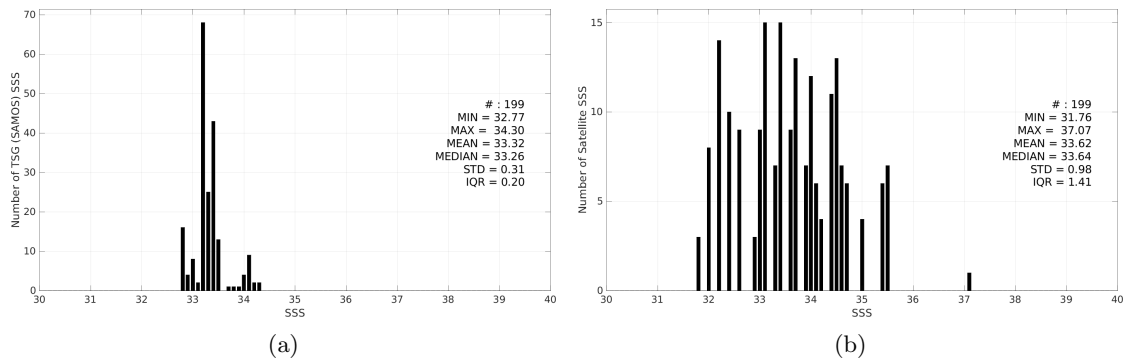
Figure 3: Histograms of SSS from TSG (SAMOS) (a) and SMAP SSS L2 v5.3 - 40 km (RSS) (b) considering all match-up pairs per bins of 0.1 over the Ganga and Brahmaputra river plumes Pi-MEP region and for the full satellite product period.
