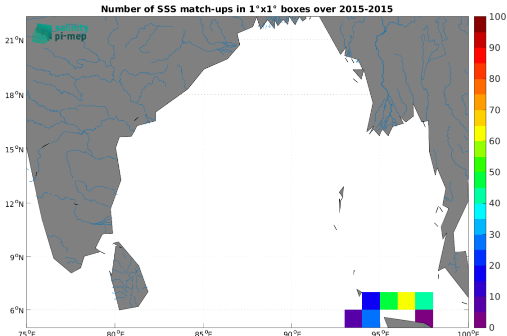
Figure 5: Number of SSS match-ups between TSG (SAMOS) SSS and the SMAP SSS L2 v5.3 - 40 km (RSS) SSS product for the Ganga and Brahmaputra river plumes Pi-MEP region over 1^\circ \times 1^\circ boxes and for the full satellite product period.
